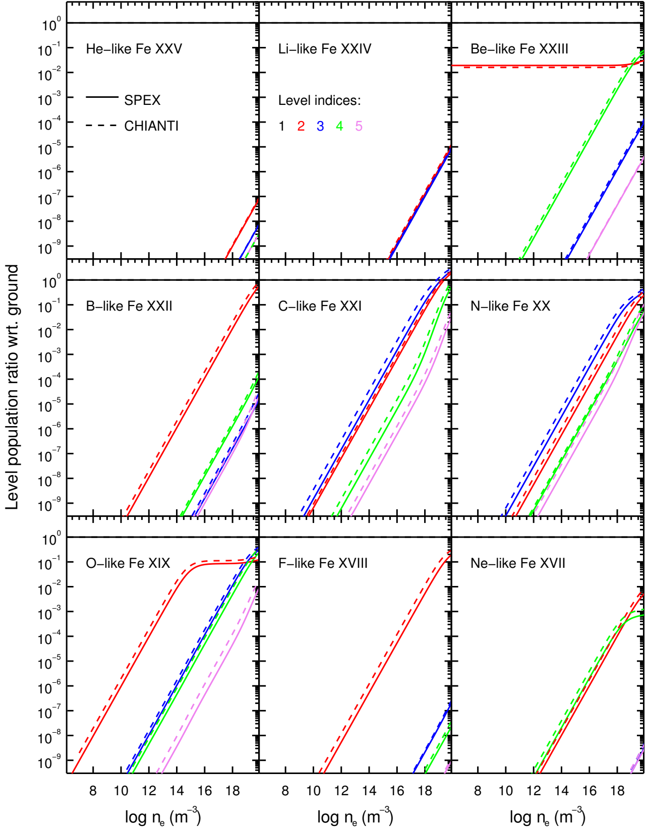
Fig. B.1. Level population ratio for the first four excited levels (level indices 2–5) of the Fe ionization sequence from He-like Fe XXV to Ne-like Fe XVII for collisional ionized equilibrium (CIE) plasma, using SPEXACT v3.04 (solid line) and CHIANTI v8.0.8 (dashed line). The CHIANTI atomic database v8.0.6 is used.
