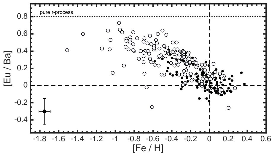
Fig. 3. [\text{Eu}/\text{Ba}] as a function of [\text{Fe}/\text{H}] . The full sample is divided into thin and thick disks according to our age-selection criterion. The dotted line represents a pure r -process ratio derived from Bisterzo et al. (2014). The average error is also presented.
