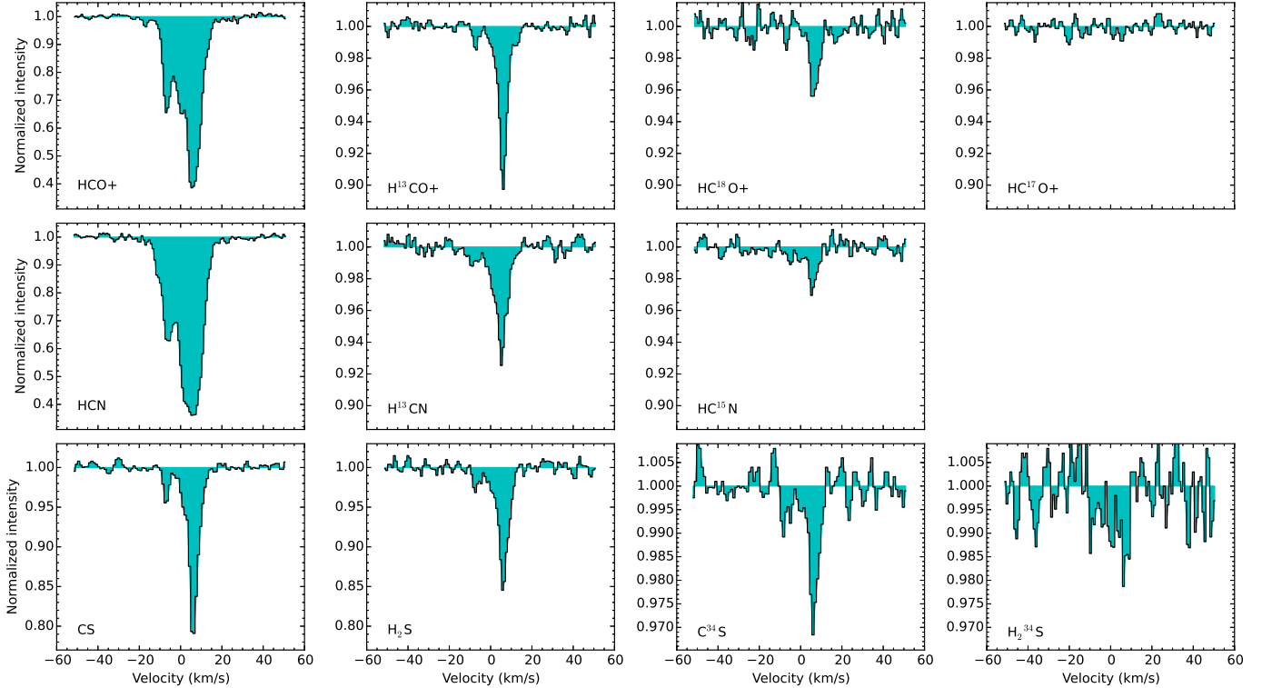
Fig. 2. Averaged spectra of the \text{HCO}^+ , \text{HCN} , \text{CS} , and \text{H}_2\text{S} isotopologues. The velocity resolution is 0.9 \text{ km s}^{-1} . The \text{HCN} spectrum is slightly broadened by the hyperfine structure.
