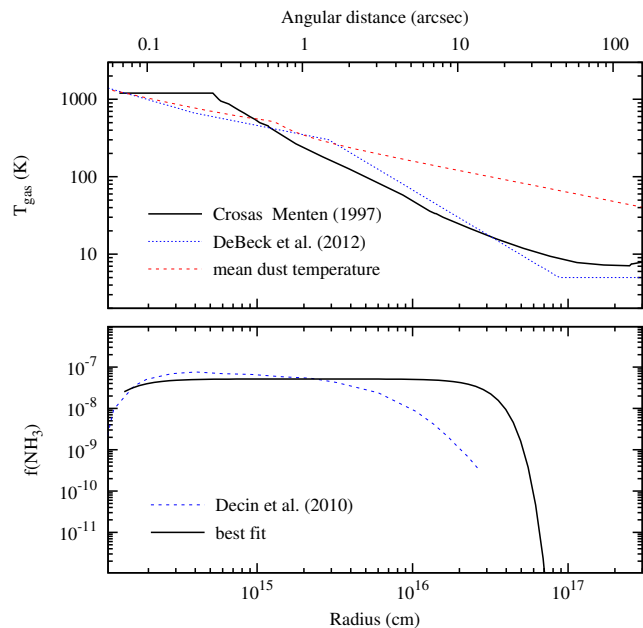
Fig. 3. Gas temperature within the envelope of IRC+10216 adopted for this work ( upper panel ) from Crosas & Menten (1997) is shown by a solid line, while that from De Beck et al. (2012) is shown by a blue dotted line. The dust temperature is shown by a red dashed line. The lower panel shows the distribution of ammonia from our best fitting models (solid line), and its theoretical distribution (dashed line) from Decin et al. (2010) . The angular distance is given in the top axis of the upper panel for an assumed distance to IRC+10216 of 130 pc.
