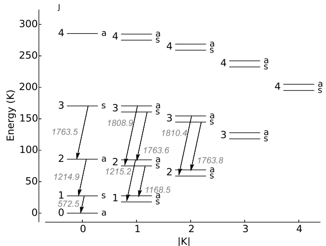
Fig. 1. Diagram of energy levels of ortho- ( |K| = 0, 3 , etc.) and para- \text{NH}_3 ( |K| = 1, 2, 4 , etc.). The inversion splitting between levels of different symmetry is exaggerated for clarity. The observed rotational transitions with frequencies in GHz are indicated with arrows.
