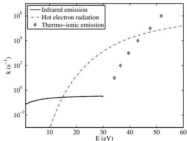
Fig. 1. Cooling rates for C 60 as a function of the internal energy of the molecule.
