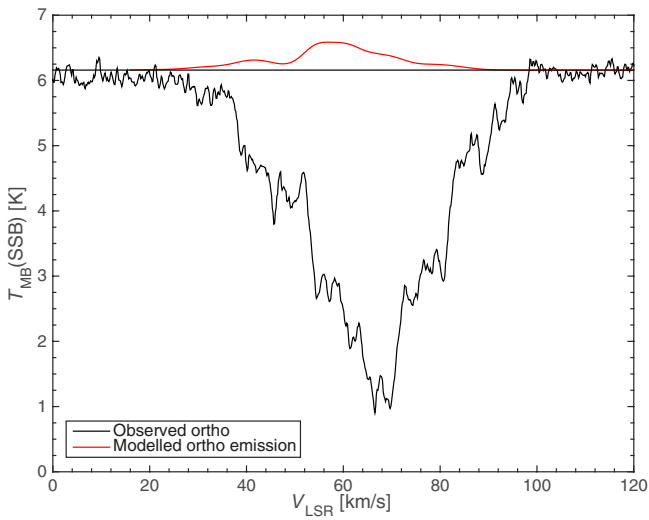
Fig. A.7. W51. Notation as in Fig. A.5.
