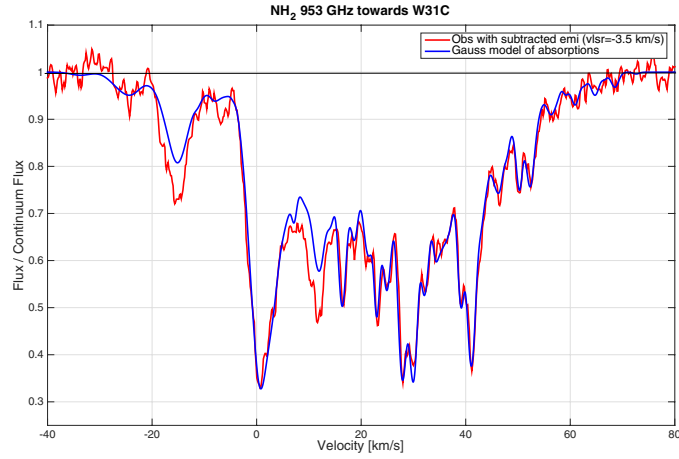
Fig. A.2. W31C. Red: original observations (channel separation 0.157 km s -1 ) with subtracted emission. Blue: Gaussian fits of all velocity (and hfs) components. Line widths and v LSR for each velocity component were taken from the results of the simultaneous Gaussian fitting of NH, ortho-NH 2 , and ortho-NH 3 (method I, described in paper II).
