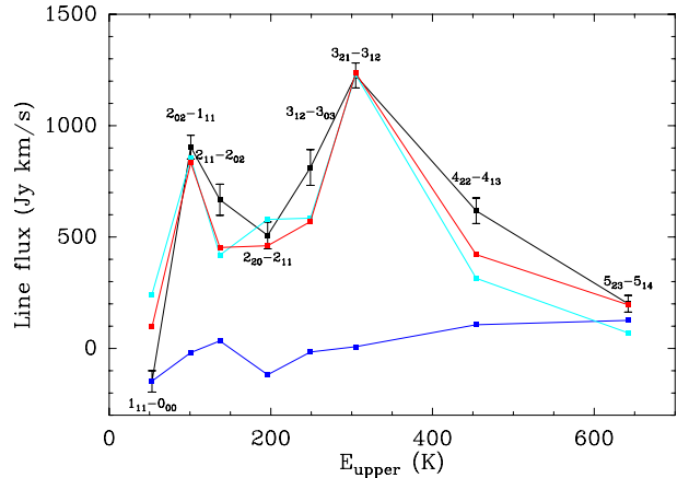
Fig. 4. Spectral line energy distribution of the H 2 O lines detected with SPIRE, the black curve represents the data. For the 1_{11} \rightarrow 0_{00} line, only the absorption part is included. The line with upper energy level 249 K is 3_{12} \rightarrow 3_{03} . Model predictions are included, the blue and light-blue curves show the contribution from C_{\text{core}} and C_{\text{outer}} , respectively. The red curve indicates the sum of the fluxes predicted by the two models.
