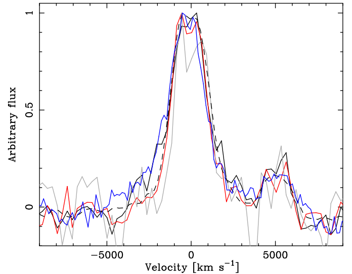
Fig. 5. Evolution of the H \alpha line profile following the 2014 eruption of M31N 2008-12a. Line colours as Fig. 3, dashed-black line indicates the H \alpha profile from the HET spectra following the 2012 eruption ( t - t_{\max} = 0.62 \pm 0.1 days; see Fig. 4). The peak redwards of H \alpha is the He I (6678 Å) emission.
