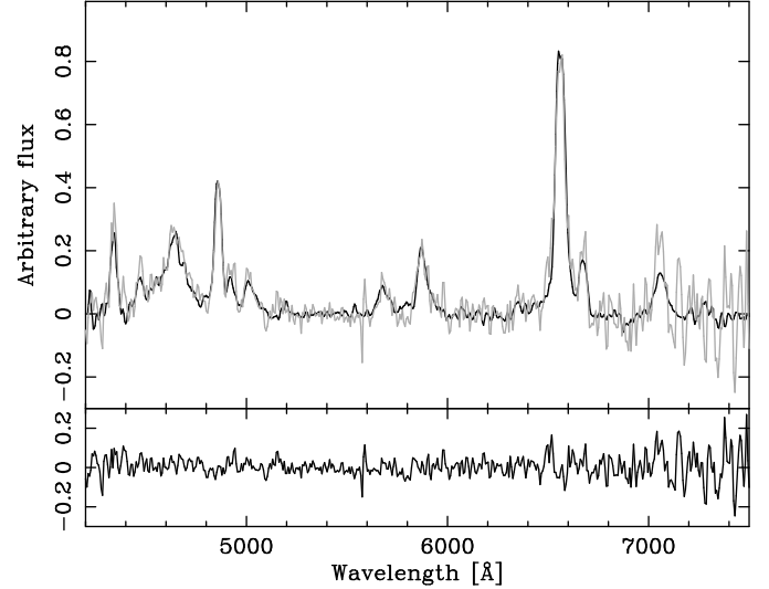
Fig. 4. Direct comparison between the HET spectrum of the 2012 eruption of M31N 2008-12a ( t - t_{\max} = 0.62 \pm 0.1 days; black line; DWB14) and the second epoch spectrum of the 2014 eruption (LT; t - t_{\max} = 0.26 days; grey line). Bottom panel: residuals following subtraction of the 2012 spectrum from the 2014 spectrum.
