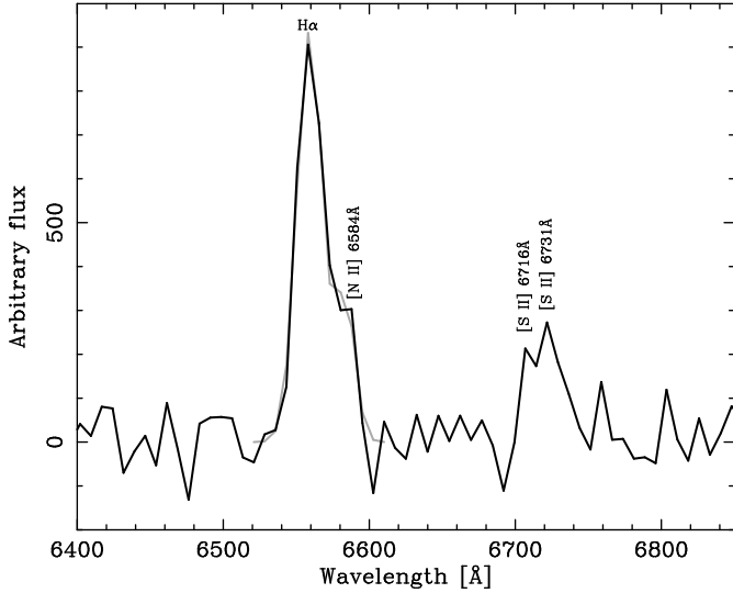
Fig. 9. Liverpool Telescope SPRAT spectrum of the apparent south-western “knot” in the extended emission around the position of M31N 2008-12a (solid black line; see also Fig. 8). The spectral range has been truncated to show only the region with significant emission; likely H\alpha , [N II] (6584 Å), and [S II] (6716 and 6731 Å) emission is labelled. The solid grey line indicates a simultaneous fit to the H\alpha and [N II] (6584 Å) emission lines.
