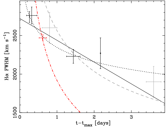
Fig. 7. Evolution of the FWHM of the H\alpha emission line following the eruption of M31N 2008-12a. Black points indicate WHT and LT spectra from the 2014 eruption, grey points are from the 2013 eruption (TBW14), and the red point is from the HET spectra in 2012 (DWB14). The solid black line shows a simple linear least-squares fit to the 2012, 2013, and 2014 data (gradient = -280 \pm 50 \text{ km s}^{-1} \text{ day}^{-1} ), the grey dashed line a power-law of index -1/3 , the red dot-dashed line a power-law of index -1/2 , and the black dotted line the best fit power-law with index -0.12 \pm 0.05 , see the text for details.
