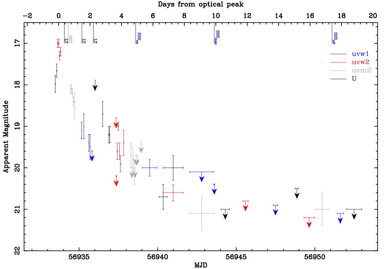
Fig. 2. Swift UV light curve of the 2014 eruption of M31N 2008-12a, all data are taken from Table 8. Here we assume optical maximum light occurred at 2014 Oct. 3.7 UT (see discussion in Sect. 4.1). Epochs of optical spectra from the 2014 eruption (black lines), 2012 eruption (grey line), and the SSS behaviour (blue lines) are shown for informational purposes.
