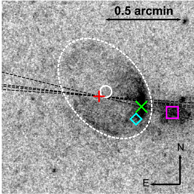
Fig. 8. LT H\alpha image ( r' -band continuum subtracted and inverted) showing the \sim 1.3 \times 1.3 region around the position of M31N 2008-12a (indicated by the red cross). The white circle, green \times , and magenta box indicate the catalogue positions of the centre of H II regions, and the blue diamond the position of a star cluster (see text in Sect. 5 for details). The white-dashed ellipse (semi-major axis 0.375 ) borders the elliptical nebulousity (semi-major axis 0.3 ) around M31N 2008-12a and is to aid the reader. The position of the south-western knot is also indicated by the green \times . The four black dashed lines indicate the slit position of the four SPRAT spectra that include emission from the SW knot (see Sect. 5.2).
