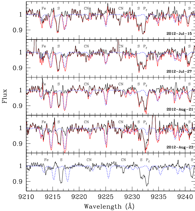
Fig. 1. Top four panels: spectra of the star ET0048, for the dates of observation, in the rest frame of the Earth, before (red) and after (black) telluric correction. Bottom panel: the final telluric-corrected, co-added spectrum, in the rest frame of the Sun. Blue dotted lines show the synthetic telluric spectra.
