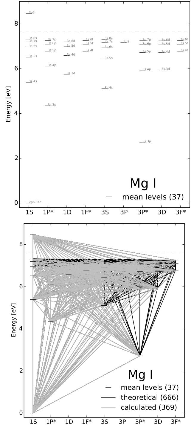
Fig. 1. Grotrian diagram of Mg I with mean energy levels labeled ( top ) and with the collision transitions ( bottom ). Theoretical collision transitions are shown with black lines whereas the calculated ones are shown with grey lines.
