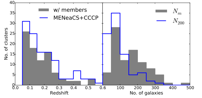
Fig. 1. Left: redshift distributions of all MENeACS+CCCP clusters (blue histogram) and clusters used in this study (gray filled histogram). Right: distributions of number of spectroscopic members, N_m (gray filled histogram), and number of spectroscopic members within r_{200} , N_{200} (blue histogram). Abell 2142, with N_m = 1052 and N_{200} = 731 , is not shown.
