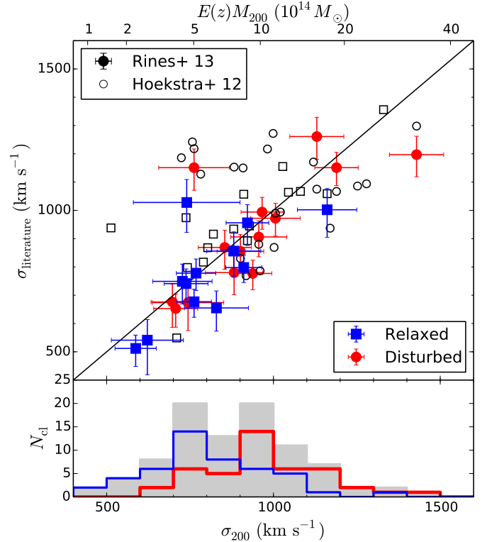
Fig. 3. Top : comparison between velocity dispersions calculated from spectroscopic members in this work with those in Rines et al. (2013) , and with velocity dispersions calculated by fitting a single isothermal sphere to the weak lensing profile ( Hoekstra et al. 2012 ) for CCCP clusters used in this work. Errorbars are not shown for the latter for clarity. Squares and circles show relaxed and disturbed clusters, respectively. The black line shows the one-to-one relation, and the top axis shows E(z)M_{200} for a given \sigma_{200} from the Evrard et al. (2008) relation. Bottom : distribution of velocity dispersions of the full sample. The gray histogram shows the total distribution, with the blue and red histograms showing the distributions for relaxed and disturbed clusters, respectively.
