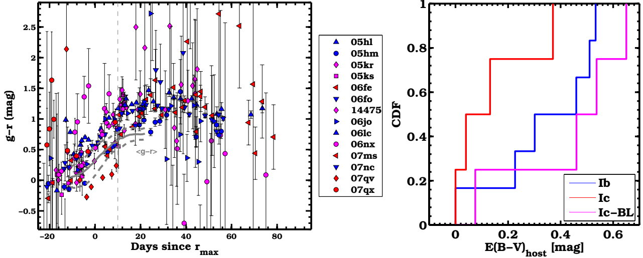
Fig. 14. Lefthand panel: g-r color (corrected only for the Galactic extinction) as a function of time since r_{\max} for 14 SDSS SNe Ib/c. The average extinction-corrected \langle g-r \rangle color of seven SE SNe (see Sect. 3.3.1 for details) is shown by a solid gray line. Its value at 10 days (this epoch is labeled by a vertical dashed gray line, where g-r = 0.64 \pm 0.13 mag) is assumed as the intrinsic colour for computing the host extinction for each SN. A Cardelli et al. (1989) reddening law with R_V = 3.1 is adopted in the computation. Righthand panel: cumulative distribution functions of E(B-V)_{\text{host}} for SNe Ib, Ic, and Ic-BL. The corrections for SNe Ib and Ic-BL appear larger than those needed for SNe Ic. The uncertainty on each E(B-V)_{\text{host}} is 0.2 mag.
