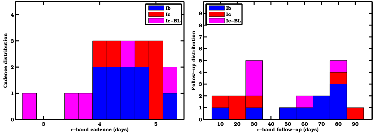
Fig. 7. Left hand panel: r-band cadence distribution for the SDSS SN Ib/c sample. Typical values are between 4 and 5 days. Righthand panel: r-band follow-up distribution for the SDSS SN Ib/c sample. SNe were followed for a minimum of \sim 10 days to a maximum of \sim 90 days after discovery.
