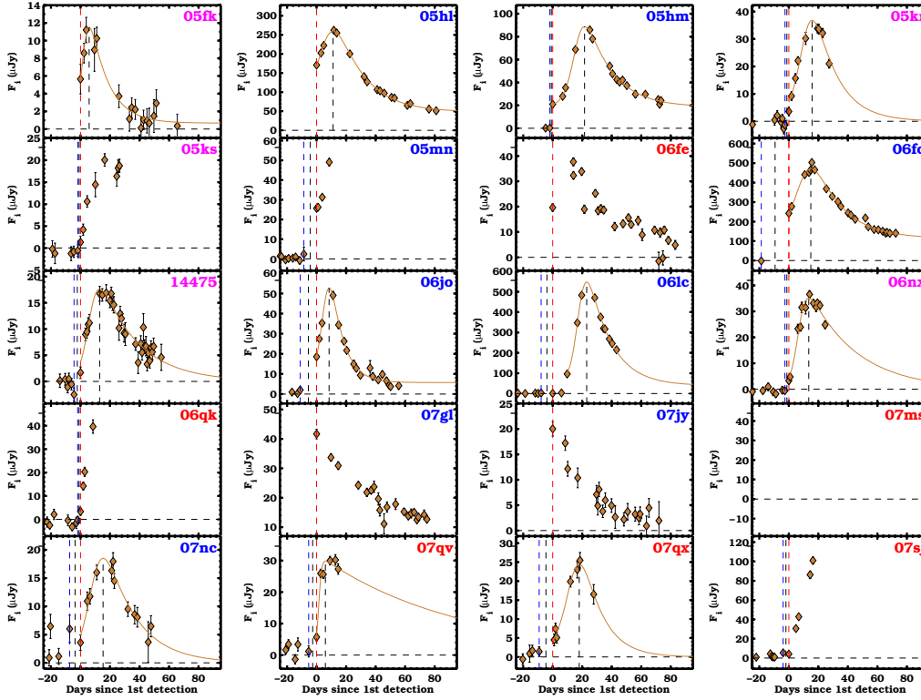
Fig. 5. i -band light curves of 20 SDSS SNe Ib, Ic, and Ic-BL. Best fits on the SN light curves observed before peak are shown by a dark yellow solid line. Vertical blue and red dashed lines mark the last non-detection and the first detection epoch. Vertical black dashed lines indicate the derived explosion date and the peak epoch. Light curves are shown after correction for time dilation. Blue, red, and magenta labels correspond to SNe Ib, Ic, and Ic-BL, respectively.
