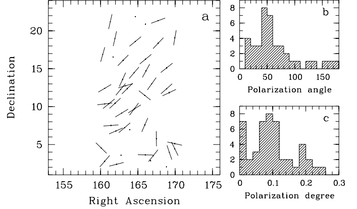
Fig. 2. Interstellar polarization in the region of the sky corresponding to the quasar large-scale structure under study (data from Berdyugin et al. 2014). a) Map of polarization vectors; right ascensions and declinations are in degree; the length of the polarization vectors is arbitrary. b) Distribution of polarization angles (in degree). c) Distribution of polarization degrees (in %).
