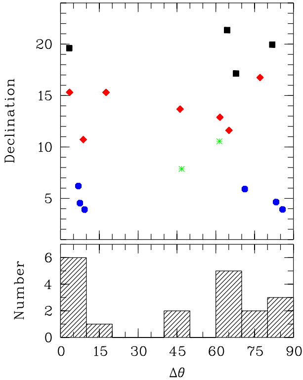
Fig. 5. Bottom: distribution of the acute angle \Delta\theta (in degree) between quasar polarizations and the orientation of their host large-scale structure. Top: \Delta\theta is plotted against the object's declination (in degree) to illustrate the behavior of the different quasar groups (1: squares; 2: lozenges; 3: asterisks; 4: hexagons; colors as in Fig. 4).
