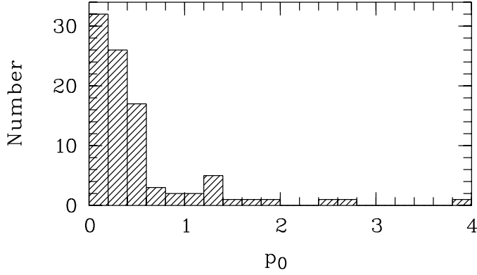
Fig. 1. Distribution of the debiased polarization degree p_0 (in %) measured for the sample of 93 quasars.
