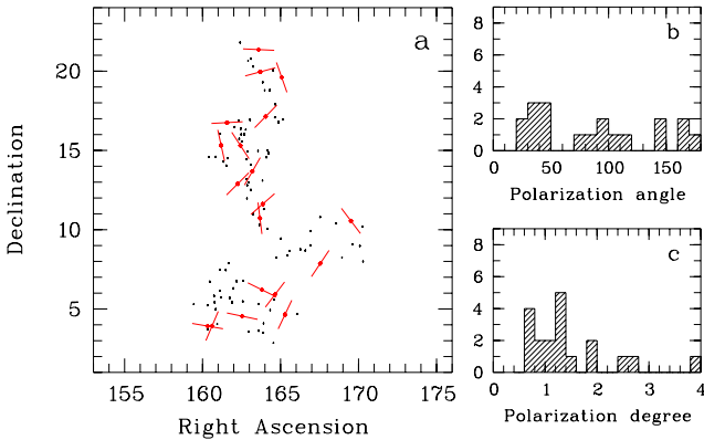
Fig. 3. Polarization of the 19 quasars with p \geq 0.6\% . a) Map of polarization vectors over the large-scale structure; right ascensions and declinations are in degree; the length of the polarization vectors is arbitrary. b) Distribution of polarization angles (in degree). c) Distribution of polarization degrees (in %).
