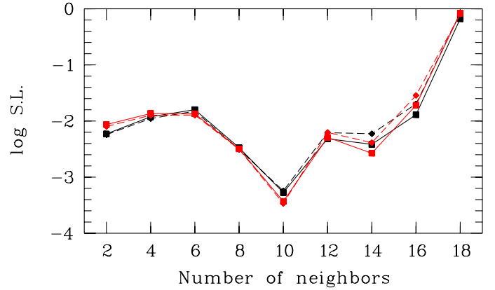
Fig. 7. Logarithm of the significance level (S.L.) of the Z_c test applied to the sample of 19 polarized quasars, as a function of the number of nearest neighbors. The solid line refers to simulations obtained by shuffling angles over positions while the dashed line refers to simulations obtained by randomly generating angles. The statistics are computed with (in red) and without (in black) parallel transport of the polarization vectors.
