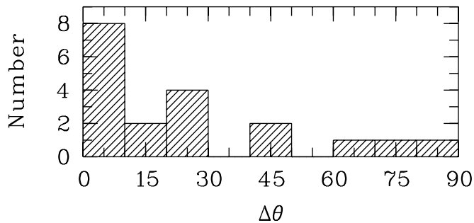
Fig. 9. Distribution of the acute angle \Delta\theta (in degree) between quasar polarizations and the orientation of their host large-scale structure after rotating by 90^\circ the polarization angles of objects with MgII emission line widths larger than 4300 \text{ km s}^{-1} .
