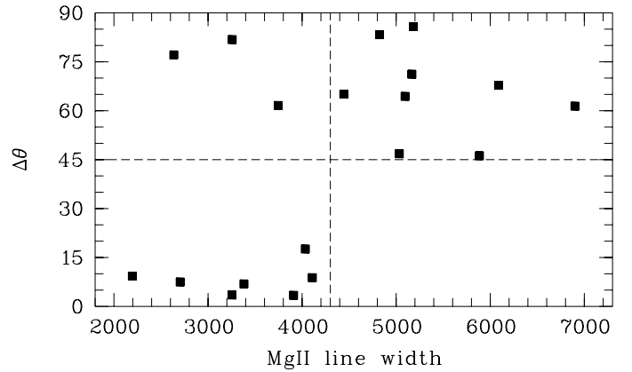
Fig. 8. Angle \Delta\theta (in degree) between quasar polarizations and the orientation of their host large-scale structures as a function of the MgII emission line width (FWHM in \text{km s}^{-1} ).
