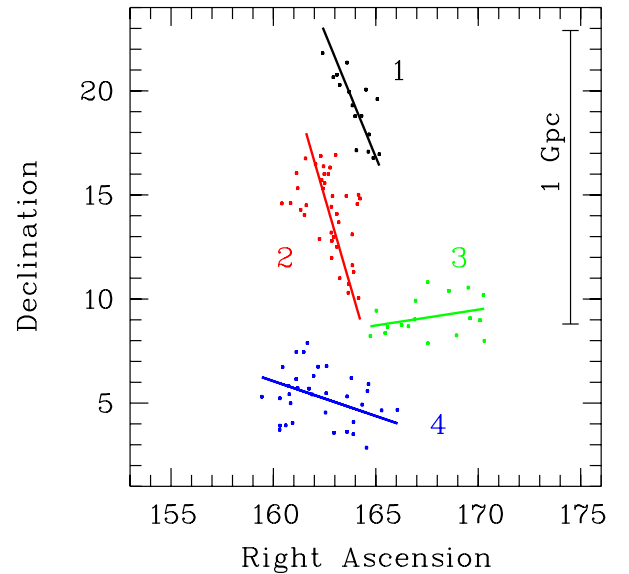
Fig. 4. Quasar groups and their orientations on the sky. Right ascensions and declinations are in degree. The superimposed lines illustrate the orientations of the four groups labeled 1, 2, 3, 4. The comoving distance scale at redshift z = 1.3 is indicated assuming a flat Universe with H_0 = 70 \text{ km s}^{-1} \text{ Mpc}^{-1} and \Omega_m = 0.27 .
