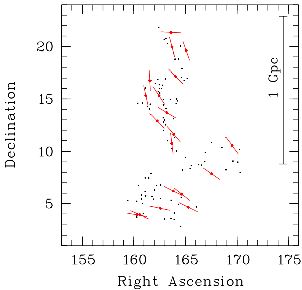
Fig. 6. Polarization vectors of the 19 quasars with p \geq 0.6\% are superimposed on the large-scale structure after rotation of the polarization angles according to \tilde{\theta} = \text{mod}(\theta, 90^\circ) + 90^\circ . A clear correlation is seen but we nevertheless caution against exaggerated visual impression since polarization angles are now in the range [90-180^\circ] . Right ascensions and declinations are in degree. The comoving distance scale is indicated as in Fig. 4.
