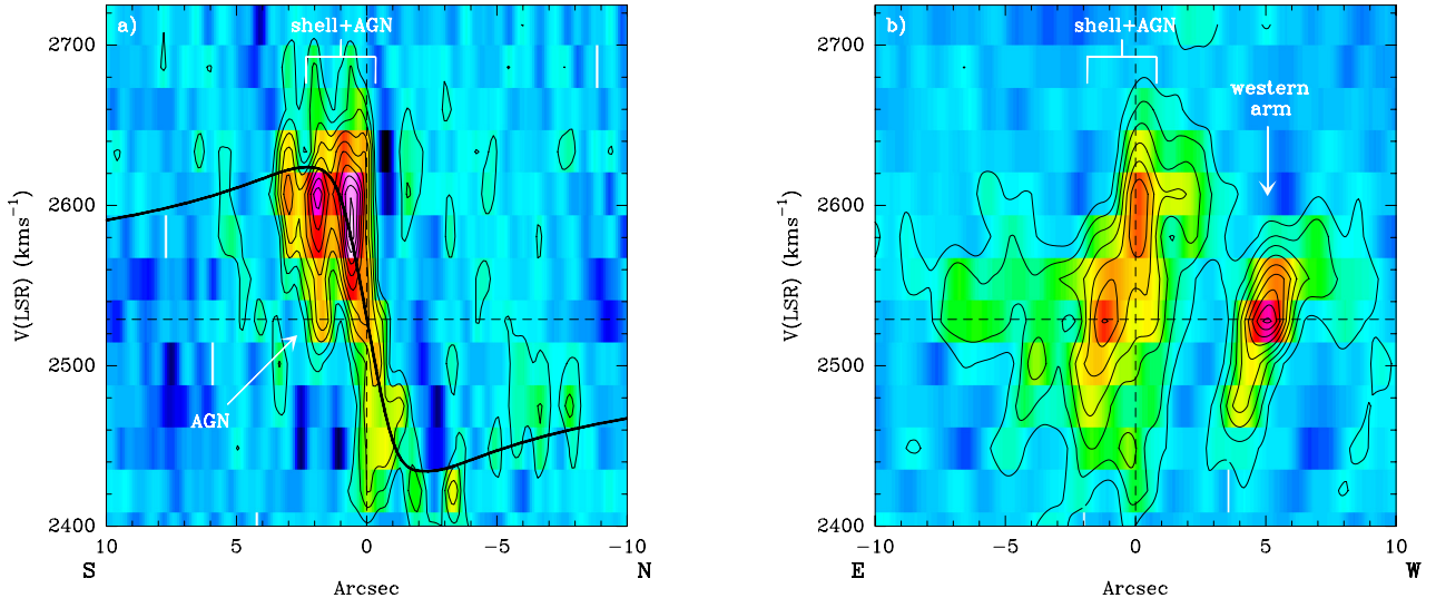
Fig. 3. CO 2–1 position-velocity diagrams along the major (north-south, left ) and the minor (east-west, right ) axes of the NGC 4194 obtained from the high-resolution data cube within a slit width of 1'' . The contour levels start at 1.5\sigma in steps of 1.5\sigma . The colors range from 0 to 0.1 \text{ mJy/beam} . The result of the fitted Brandt rotation curve, using a fixed inclination value of 40^\circ , is shown on the left .
