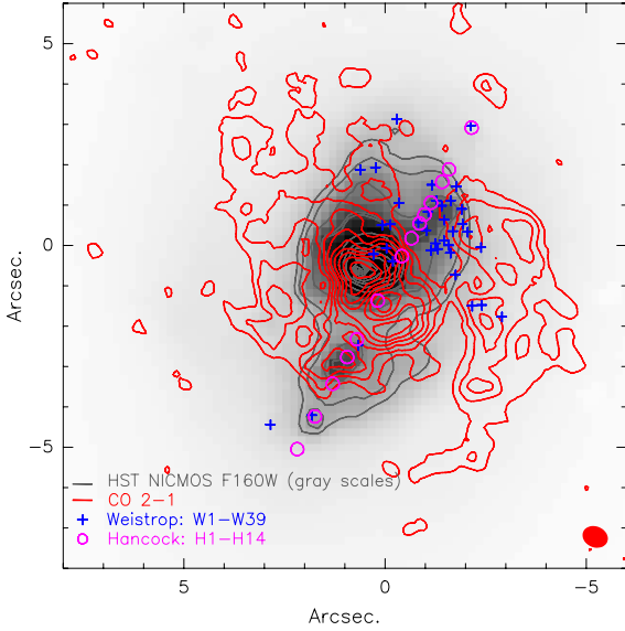
Fig. 8. Overlay of the ^{12}\text{CO} 2-1 emission contours on top of an HST WFPC2 F606W filter image. North is up, east to the left. Blue crosses indicate the positions of the star clusters that were found by Weistrop et al. (2004) in the UV; magenta circles represent the star clusters identified in the visible (Hancock et al. 2006). The CO beam size is indicated in the lower right corner.
