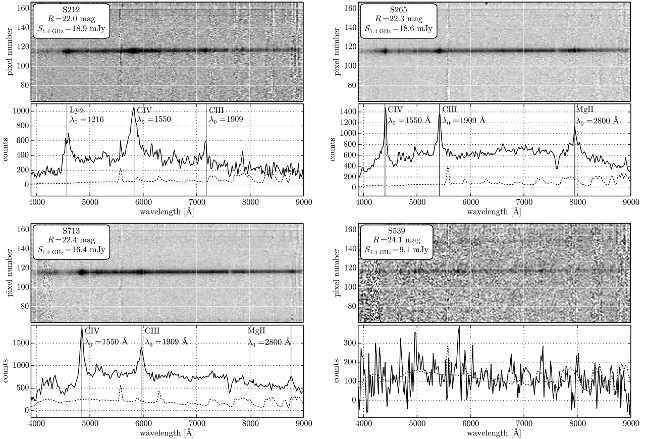
Fig. 1. Spectra of IFRS S212 (upper left), S265 (upper right), S713 (lower left), and S539 (lower right). For each IFRS we show the two-dimensional spectrum (upper plot) and the extracted one-dimensional spectrum (lower plot). We list the ID, the R band Vega magnitude, and the 1.4 GHz radio flux density of each IFRS. In the one-dimensional spectrum, the solid line represents the spectrum of the IFRS while the dotted line shows the sky background in arbitrary units. Additionally, the position of emission lines are marked by vertical lines for a redshift of z = 2.76 (S212), z = 1.84 (S265), and z = 2.13 (S713).
