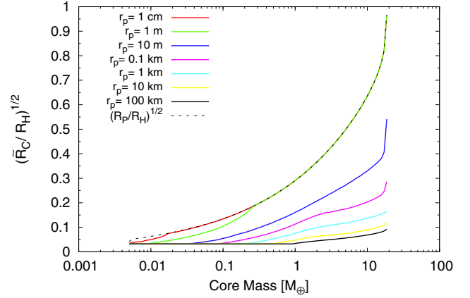
Fig. 15. Factor \sqrt{R_C/R_H} as a function of the core mass for different planetesimal sizes. The plot corresponds to the case of a disk ten times more massive than the MMSN and r_p^{\max} = 100 km when planetesimal coagulation and fragmentation are considered. The black dashed line corresponds to the evolution of the term (R_p/R_H)^{1/2} , where R_p is the radius of the planet. (Color version online.)
