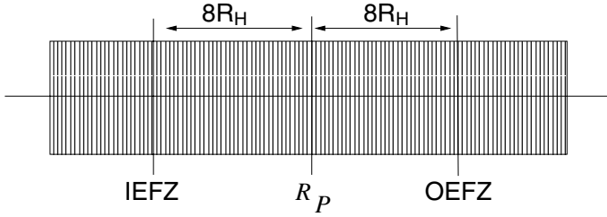
Fig. 1. Schematic illustration of the fragmentation zone for an isolated planet in the radial grid. IEFZ (OEFZ) represents the inner (outer) edge of the fragmentation zone, while R_p is the radial bin corresponding to the planet. The fragmentation zone extends to eight Hill radii on either side of the planet.
