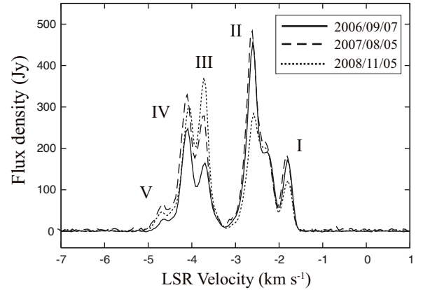
Fig. 1. Spectra of the 6.7 GHz methanol maser in Cep A obtained with the Yamaguchi 32-m radio telescope. Solid, dashed, and dotted lines show the spectra observed near in time to the VLBI epochs 1, 2 and 3, respectively. The roman numerals I–V identify different spectral features.
