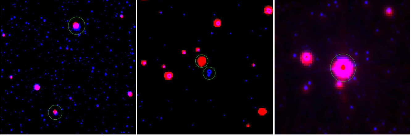
Fig. 1. Examples for the co-moving companion search. North is up and east is left. The red images are 2MASS K_S , and the blue images are VVV K_S . The objects of interest are circled. From left to right : LP 922-16 A and B ( \sim 2 \times 2 arcmin), LHS 3188 A and B ( \sim 1.5 \times 1.5 arcmin), and C* 1936 ( \sim 1 \times 1 arcmin).
