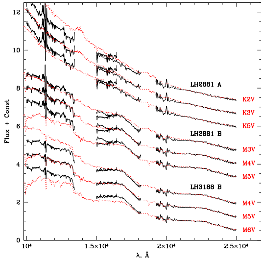
Fig. 3. Spectral classification example. Solid lines show our spectra, and dotted lines—the template spectra from the IRTF library (Cushing et al. 2005; Rayner et al. 2009).
