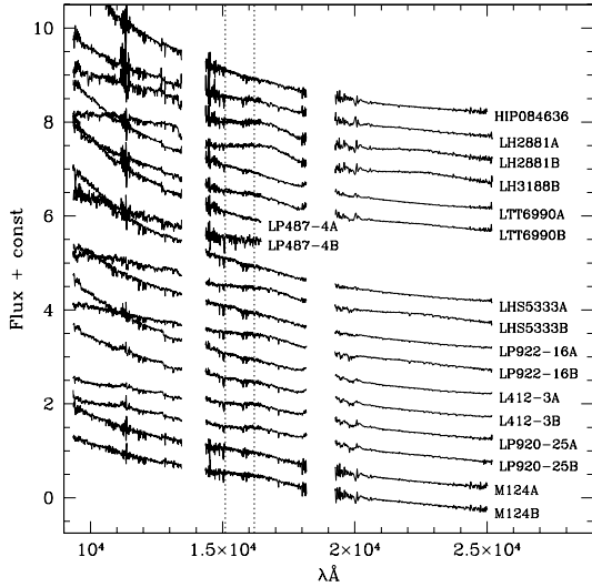
Fig. 2. Near-infrared spectra of our targets. The spectral areas with poor atmospheric transmission are omitted. The spectra were normalized to 0.5 in the overlapping region (bracketed with dotted lines) and shifted vertically by 0.5 for clarity. M124A and M124B indicate MACHO 124.22158.2900 and MACHO 124.22158.2910, respectively; L412-3 B is an alternative notation of HD 322416 and LP920-25 B is the same for LP920-26. The spectrum of the telluric HIP 084636 shown here was corrected for the atmospheric absorption with HIP 098813.
