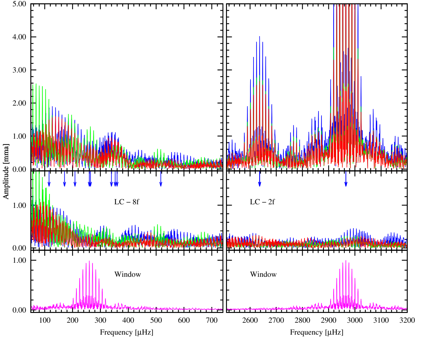
Fig. 7. Amplitude spectrum of the orbit-subtracted Ultracam light curve (LC), for the two frequency regions where pulsations are observed. Upper panel: the amplitude spectra of the three photometric channels (red: r -band, green: g -band, blue: u -band). Middle panel: the same spectra after prewhitening the 10 frequencies listed in Table 6 from the LC. Lower panel: window function for the two frequency regions.
