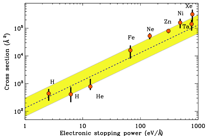
Fig. 3. Experimentally measured OH-db destruction (porosity loss) cross sections as a function of the stopping power in eV/Å. The dotted line corresponds to the best fit cross section and the yellow coloured zone defines the boundaries for the cross section curves ( \sigma^{OH-db}(S_{[eV/\text{Å}]}) = 131_{-65}^{+170} S_{[eV/\text{Å}]}^{1.0 \pm 0.2} , see text for details).
