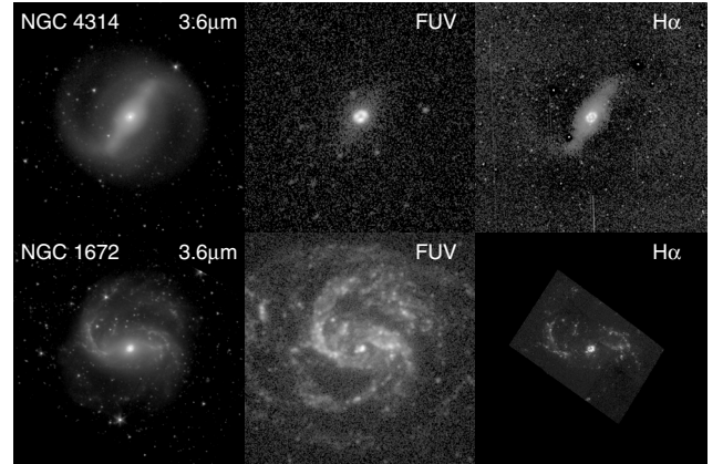
Fig. 1. NGC 4314 (top row) is an (R 1 )SB(rl,nr)a galaxy (Buta et al., in prep.) with a passive inner ring-lens. NGC 1672 (bottom row) is an (R 1 )SAB(rs,nr)b galaxy (Buta et al., in prep.) whose inner pseudoring is still forming stars. In the first case the inner feature does not emit in the FUV and H \alpha . There is a significant amount of emission in these bands for the active inner feature. The prominent ring feature in NGC 4314 is a nuclear ring. The 3.6 \mu\text{m} images are from the S 4 G, the FUV images come from GALEX’s NGS survey, and the H \alpha images come from Knapen et al. (2004) and the HLA.
