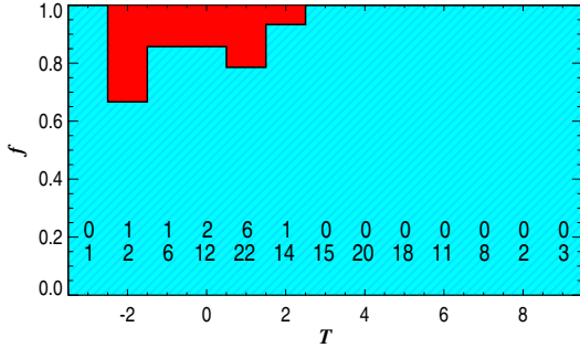
Fig. 3. Fraction of active and passive inner rings according to the FUV indicator as in Fig. 2, but now for inner rings in galaxies that have both FUV and H\alpha imaging available.
