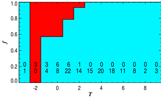
Fig. 4. As Fig. 2, but now using H\alpha emission as an indicator on whether inner rings are passive or active.
