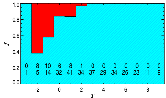
Fig. 2. Fraction of active and passive inner rings (blue hatched and red plain surfaces, respectively) according to the FUV indicator as a function of the galaxy stage for galaxies in the sample with available GALEX imaging. The bottom row of numbers indicate the number of active rings for a given stage and the top row indicates the number of those that are passive.
