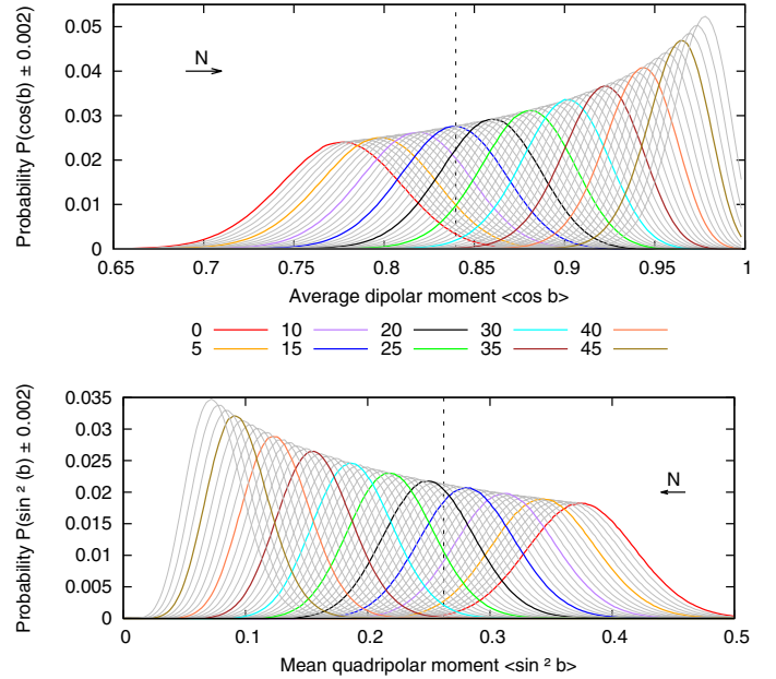
Fig. 4. Example of dipolar ( top ) and quadripolar ( bottom ) moment probability distributions for samples of 49 randomly generated sources with an increasing number ( N ) of those sources being of Galactic origin, and the observed value for sample #5 (dashed vertical line). Each line has a different amount of Galactic sources, starting with N = 0 (red), and only every fifth line was colored for easier reading.
