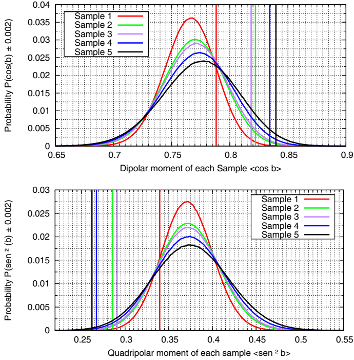
Fig. 3. Dipolar ( top ) and quadripolar ( bottom ) moment PMFs for samples of isotropically generated sources weighted by Swift 's exposure map for each sample size, and the observed values for each sample (vertical lines).
