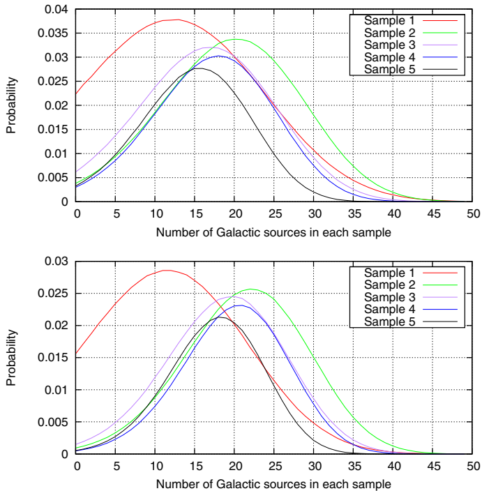
Fig. 5. Relative probability of obtaining the dipolar ( top ) and quadrupolar ( bottom ) moments \pm 0.002 measured for our samples.
