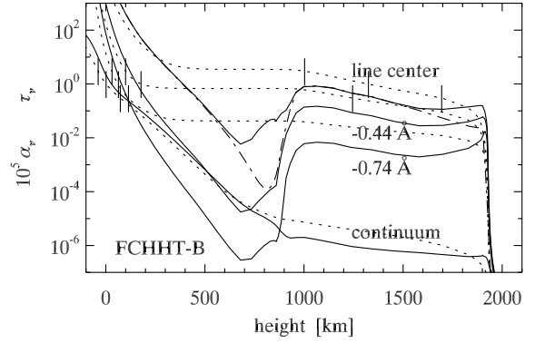
Fig. 9. Solid: H \alpha line extinction coefficients \alpha_\nu' per m against height for the FCHHT-B model, at line center and in the blue wing at \Delta\lambda = -0.44 and -0.74 \text{ \AA} , and the continuum opacity \alpha_\nu^c in the adjacent continuum. The dot-dashed curve is the line-center result for LTE. The opacities are multiplied by a scale height of 10^5 \text{ m} to make them comparable to the corresponding optical depth scales (dotted curves). The tick marks on the latter correspond to \tau_\nu = 3, 1, 0.3 . Across the opacity dip due to the temperature minimum the optical depth is \tau_\nu = 3.5, 0.7, 0.04 at the three line wavelengths, respectively.
