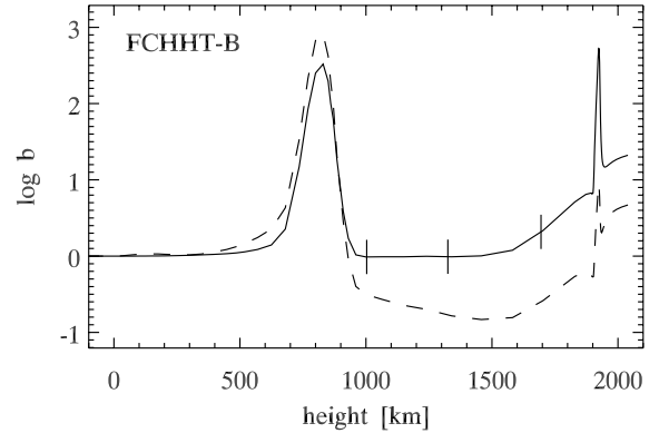
Fig. 10. H \alpha population departure coefficients against height for the FCHHT-B model. The tick marks correspond to \tau_\nu = 3, 1, 0.3 . Solid: lower-level departure coefficient b_2 . Dashed: upper-level departure coefficient b_3 .
