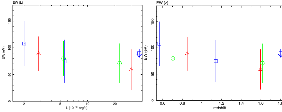
Fig. 20. Dependence of unresolved 6.4 keV Fe line equivalent width on the average luminosity ( left ) and the average redshift ( right ) of the subsamples (first row of Table 3). Squares: L-z subsamples; circles: redshift subsamples; triangles: luminosity subsamples. We represent upper limits by a down-pointing arrow. Each set of points with the same symbol are statistically independent, but not between the symbols.
