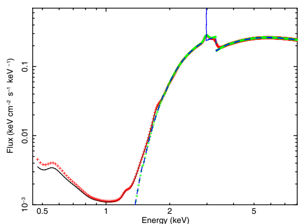
Fig. B.2. Comparison, for a simulated absorbed source, between: unfolded spectrum with best fit (green circles), with \gamma = 2 (red plus), with \gamma = 0 (continuous black line), with the model (dashed blue line).
