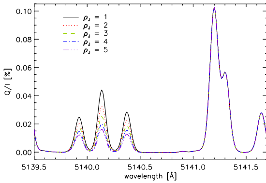
Fig. 6. When the collision rates of the R triplet are enhanced by a factor of \rho_J compared to the P triplet, the R lines show additional depolarization. These J -dependent collisions were predicted by Derouich (2006) and were necessary to obtain good fits to the observed spectra. The parameters used to produce this figure are \rho_C = 0.05 , B = 7 and \mu = 0.11 .
