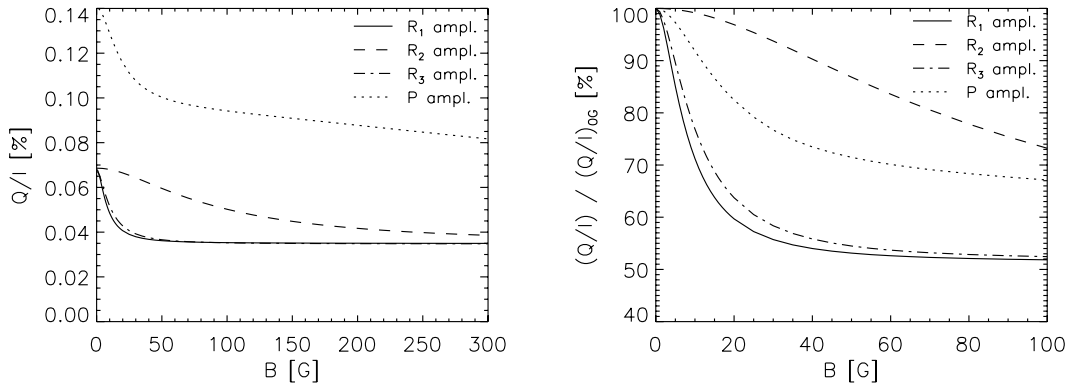
Fig. 4. Variation of the absolute Q/I including the continuum polarization with magnetic field. The parameters used for the simulation are: \rho_C = 0.05 , \rho_J = 1.5 and \mu = 0.11 . Left panel: the amplitudes of R_1 (solid) and R_3 (dash-dotted) decrease very fast and are nearly fully depolarized above 100 G. The critical field strengths of R_2 (dashed) and P (dotted) are higher. Right panel: magnification of the region from 0 G to 100 G. The y-axis is scaled with the zero magnetic field Q/I value, i.e. shows the amplitude decrease in percent. Because the continuum polarization is included and not only the line polarization is shown, the ratio does not necessarily decrease to 20% for high B .
