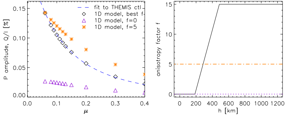
Fig. 5. Left panel: the dashed line represents the P amplitude fit to the center-to-limb THEMIS and IRSOL measurements from Paper I. Calculations with a constant anisotropy factor f cannot reproduce these amplitudes (asterisks for f = 5 and triangles for f = 0 ). The right panel shows the corresponding height dependence of f (dash-dotted line for f = 5 and dotted line for f = 0 ). It was varied linearly (solid line, right panel ), which created a good fit to the measured P amplitudes (diamonds, left panel ).
