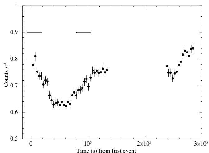
Fig. 1. Lightcurve of the Chandra observations. The solid horizontal lines mark the HST-COS observation intervals.
