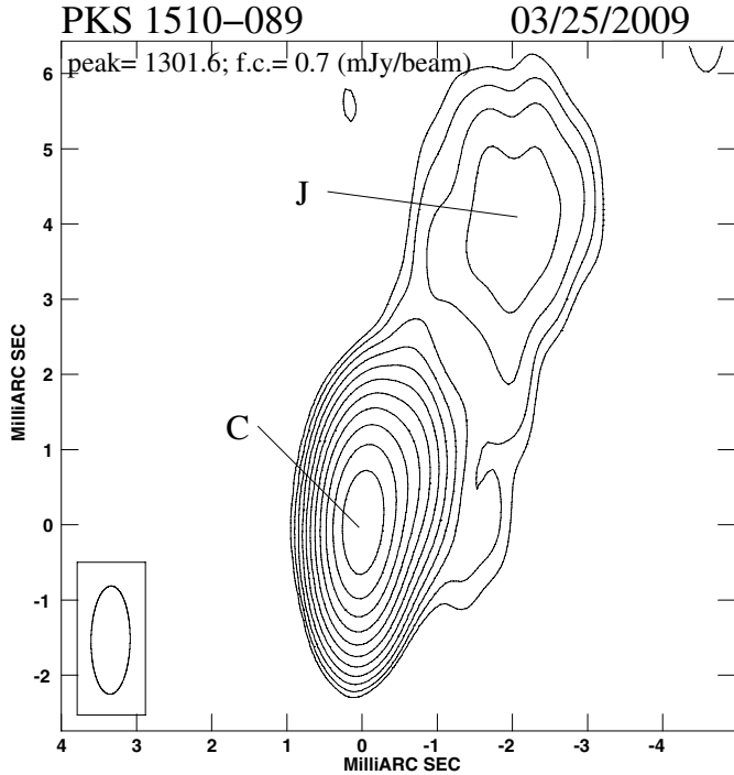
Fig. 5. VLBA image at 15 GHz of PKS 1510–089 on 25 March 2009. On the image we provide the restoring beam, plotted in the bottom left corner, the peak flux density in mJy beam -1 , and the first contour (f.c.) intensity in mJy beam -1 , which is 3 times the off-source noise level. Contour levels increase by a factor of 2.
