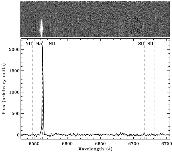
Fig. 4. A zoom-in of the optical spectrum covering H\alpha and the [N II] and [S II] line doublets. The weakness of [N II] and [S II] relative to H\alpha indicate that this object is a PN and not a SNR (see Sect. 4 for details). The top panel shows the two-dimensional spectrum at corresponding wavelengths (white pixels indicate large, positive pixel values). The slit height measures 12'' , while the spatial extent of the resolved H\alpha is about 6'' .
