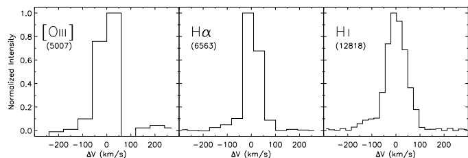
Fig. 5. A sample of the narrow emission lines present in the X-shooter spectra: [O III] ( left ) at 5007 Å, H \alpha ( middle ) and H I (Pa \beta , right ) at 12818 Å.
