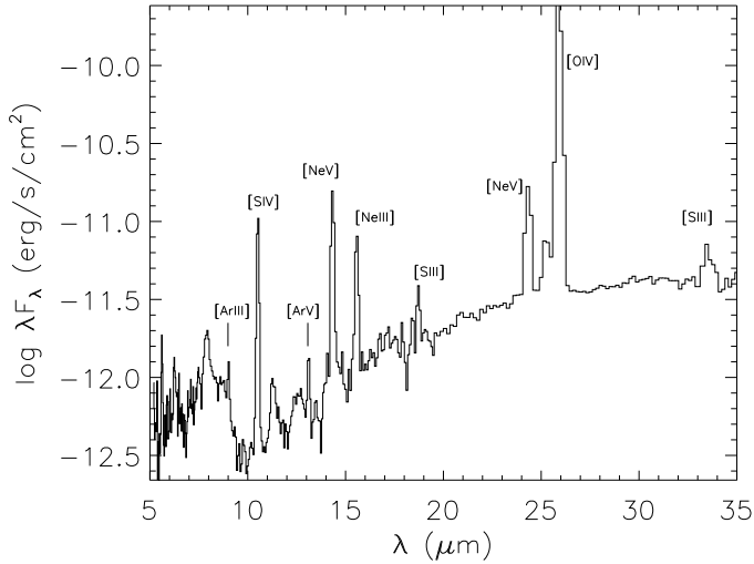
Fig. 1. IRS spectrum of OL17, a PN/SNR candidate found among the sample from Oliveira et al. (2010). The [O IV] line (25.89 \mu\text{m} ) clearly dominates the spectrum.
