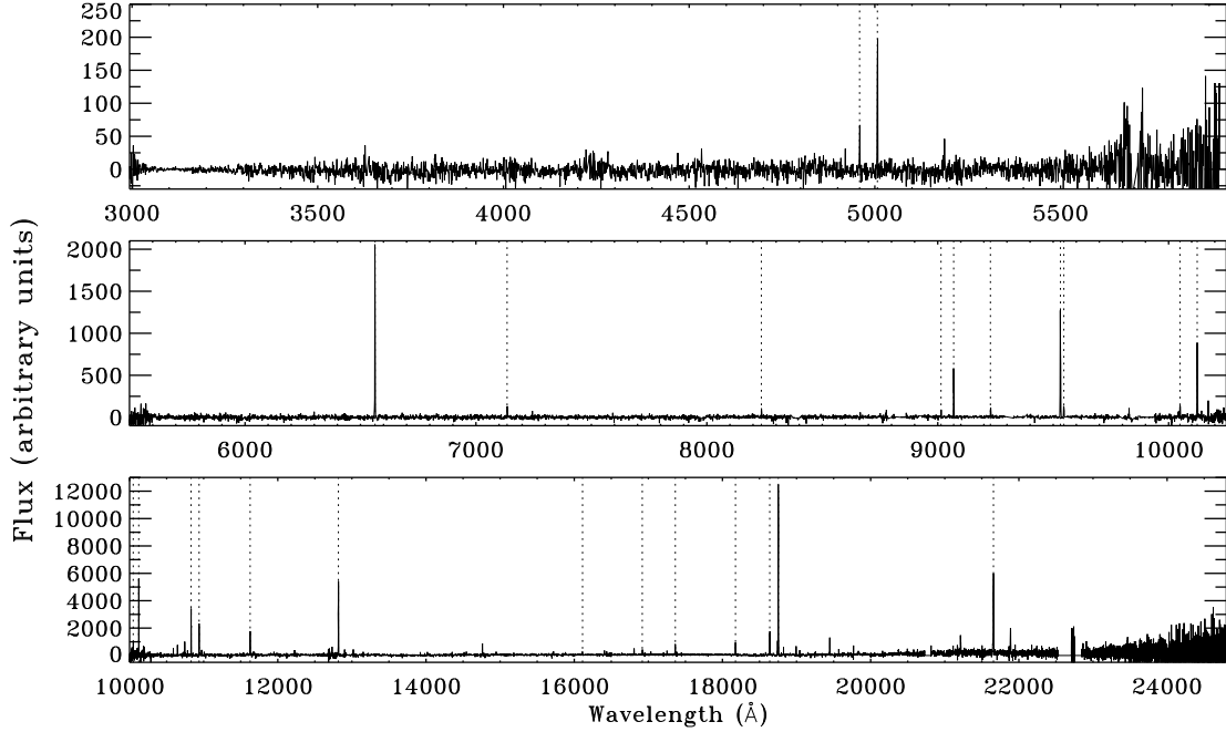
Fig. 3. X-shooter spectra of OL17. Panels show the one-dimensional spectra extracted from the UV/blue ( top ), the visible ( middle ), and the near-infrared ( bottom ) arms. Dotted lines mark the major emission lines tabulated in Table 3.
