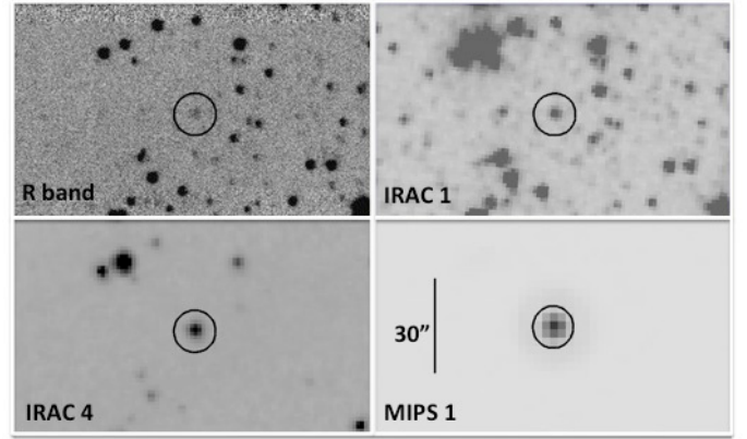
Fig. 2. Optical and infrared images showing the INT/WFC R -band (top-left), IRAC1 (top-right), IRAC4 (bottom-left) and MIPS1 (bottom-right). All three images display the same field of view and a length scale of 30” is shown for reference.
