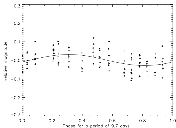
Fig. 7. Lightcurve resulting from the relative photometry. The relative magnitude is plotted versus the rotational phase (normalized to 1 rather than 2\pi ). A sinusoidal fit is superimposed.
