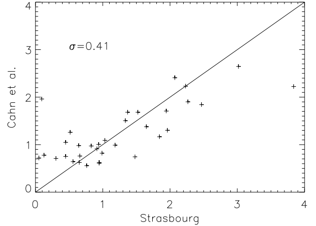
Fig. 1. c_\beta measurements by Cahn et al. (1992) plotted against data in Acker et al. (1992). The dispersion is around 0.4 in c_\beta .
