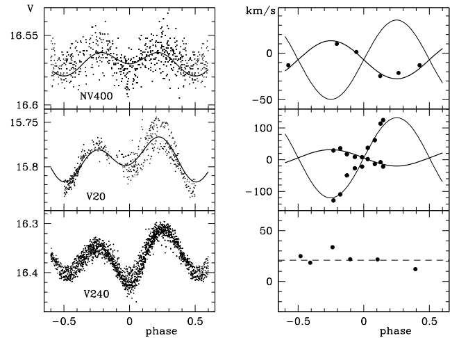
Fig. 4. Light and velocity curves of blue stragglers – continuation of Fig. 3. A single spot 2% hotter than the photosphere was placed on the primary of V20 in order to qualitatively account for the asymmetry of the light curve (just for illustrative purposes; it was not included while analyzing the data). Parameters of the fits for NV400 and V20 are given in Tables 8 and 11 in the rows indicated with an asterisk. No fit is possible for V240, because the velocity amplitude is smaller than the observational errors.
