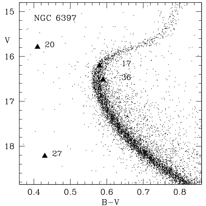
Fig. 2. Color-magnitude diagram of NGC 6397 (after Kaluzny et al. 2006 ) with marked positions of the investigated systems.
