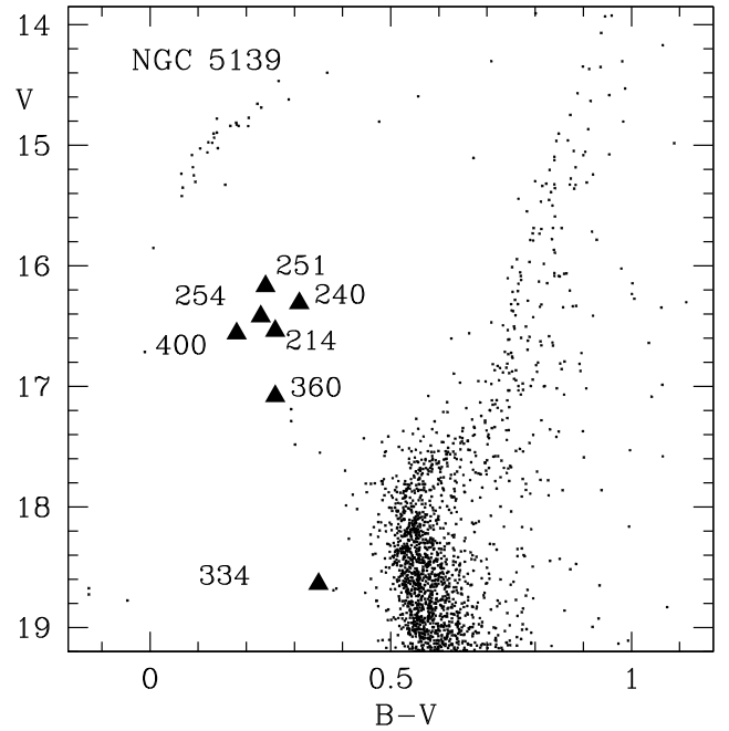
Fig. 1. Color-magnitude diagram of \omega Cen based on CASE data ( Kaluzny et al. 2004 ) transformed to the BV system with the help of standards listed by Stetson (2000) . Marked are the locations of the investigated systems.
