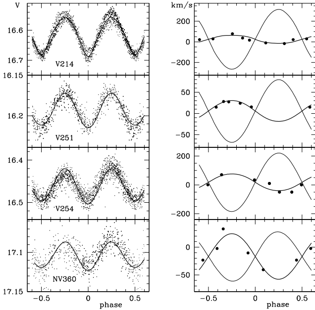
Fig. 3. Light and velocity curves of blue stragglers. Parameters of the plotted fits are given in Tables 3–5, and 7, in the rows indicated with an asterisk.
