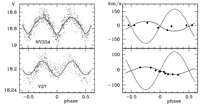
Fig. 5. Light and velocity curves of subdwarfs. Parameters of the plotted fits are given in Tables 6 and 12 in the rows indicated with an asterisk.
