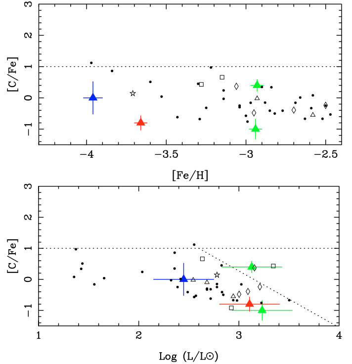
Fig. 8. DART dSph targets are in colored triangles: Sextans(Green) ScI(Blue) Fnx (Red). Other symbols are squares (Ursa MajorII), triangles (Coma Berenices), diamonds (Draco), star (Boötes) (Fulbright et al. 2004; Koch et al. 2008a; Frebel et al. 2010b; Cohen & Huang 2009; Norris et al. 2010). Only mixed Milky Way halo stars (black dots) are considered (Cayrel et al. 2004; Cohen et al. 2008; Honda et al. 2004; Aoki et al. 2005, 2007; Cohen et al. 2006; Lai et al. 2008). The dashed line delineates the regions in which they are observed.
