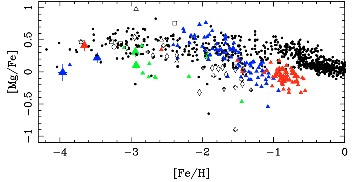
Fig. 9. DART dSph targets are in colored triangles: Sextans (Green) Sc1 (Blue) Fnx (Red). Large symbols stand for the sample stars of this work, small ones stand for earlier works and publications (Hill et al., in prep.; Letarte et al. 2010; Frebel et al. 2010a; Aoki et al. 2009; Shetrone et al. 2001). Other symbols are squares (Ursa Major II, Frebel et al. 2010b), triangles (Coma Berenices, Frebel et al. 2010b), diamonds (Draco, Shetrone et al. 2001; Fulbright et al. 2004; Cohen & Huang 2009), star (Boötes, Norris et al. 2010), cross (Carina, Shetrone et al. 2003; Koch et al. 2008a), and circle (Leo IV, Simon et al. 2010). All Milky Way halo stars from our comparison sample are considered (black dots) Cayrel et al. (2004); Honda et al. (2004); Aoki et al. (2005, 2007); Cohen et al. (2006, 2008); Lai et al. (2008). For the purpose of this figure, Venn et al. (2004)'s compilation was added at [Fe/H] ≥ -2.5.
