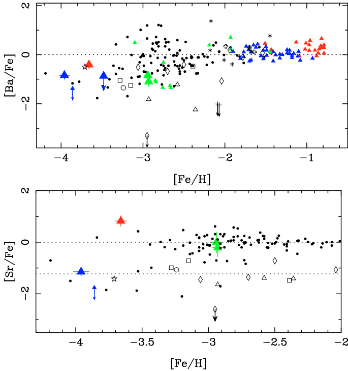
Fig. 14. Abundance ratios [\text{Ba}/\text{Fe}] and [\text{Sr}/\text{Fe}] as a function of [\text{Fe}/\text{H}] . General symbols are as in Fig. 9. From our initial comparison sample, we only keep the r -process only stars in the [\text{Ba}/\text{Fe}] plot. This requires to have measurements of the Eu abundance. This was possible with Lai et al. (2008); François et al. (2007); Honda et al. (2004); Aoki et al. (2005). We also inserted the sample of Milky Way halo stars of Barklem et al. (2005), similarly excluding carbon-rich and [\text{Ba}/\text{Eu}] > 0 ( s -process enriched stars). As to the UFDs, we use the analysis and upper limits in [\text{Ba}/\text{Fe}] of Koch et al. (2008b) on Hercules (plus sign). In the case of Scl07-49, we could only estimate an upper limit for [\text{Ba}/\text{H}] in that we indicate with an arrow. Missing the blue part of its spectrum we could not measure its abundance in SrII. Data from Shetrone et al. (2001) in Ursa Minor are identified with small six-branches stars and. The Carina stars (crosses) at [\text{Fe}/\text{H}] > -2.5 are taken from Shetrone et al. (2003). The dotted line at [\text{Sr}/\text{Fe}] = -1.23 corresponds to the mean abundance ratio of the smallest dwarfs (fainter than Draco) and to the level of the Galactic halo stars for [\text{Fe}/\text{H}] \leq -3.7 .
