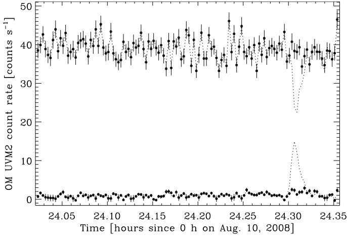
Fig. A.1. UV light curves for EX Lup (top, with the background subtracted) and for the background ( bottom ) during the S415 exposure of the OM in the fast mode. The dotted lines show the light curves obtained with the SAS script omfchain and no tracking history file. The data points show the corrected light curves using our spacecraft drift estimates. The interval of the time bin is 10 s.
