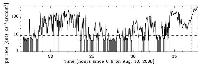
Fig. 2. Flaring-background light curve in the pn detector during our XMM-Newton observation of EX Lup. The line is the background light curve produced by the SAS task epchain . The horizontal dashed line indicates the maximum level of flaring-background for our spectral analysis. The resulting time periods with low flaring-background are shown in grey. The vertical dotted line indicates the end of the useful exposure.
