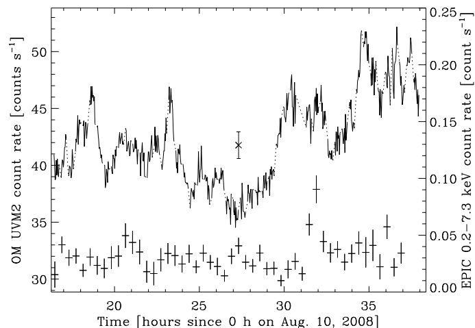
Fig. 5. Simultaneous UV and X-ray light curves of EX Lup. The upper and lower curves are the OM light curve ( left y-axis ) and the EPIC light curve ( right y-axis ), respectively. The UV light curve obtained with the OM fast mode was rebinned to bin size of 120 s. In the figure center, the cross with error bar indicates the median value and median error of the UV photometry. To guide the eye, the dotted lines link consecutive OM exposures. The bin size of the X-ray light curve is 500 s.
