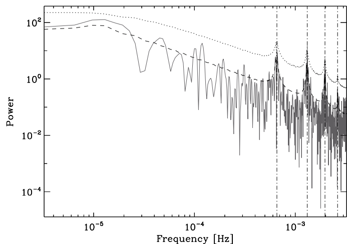
Fig. 6. Lomb normalized periodogram (LNP) of the UV light curve. The grey line is the LNP of the OM light curve. The dashed and dotted lines are the average value and the 3\sigma upper threshold of the LNP of red noise with power-law index of 1.39. The vertical dashed-dotted lines indicate the frequency associated with our observing set-up and harmonic values ( n = 2, 3, 4 ).
