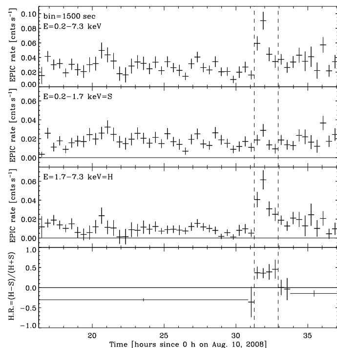
Fig. 3. XMM-Newton /EPIC background-subtracted X-ray light curves of EX Lup. The top panel shows the EPIC (pn+MOS1+MOS2) X-ray light curve of EX Lup in the energy band from 0.2 to 7.3 keV. The middle panels show the soft ( S = 0.2 –1.7 keV) and hard ( H = 1.7 –7.3 keV) band X-ray light curves. The bin size of the X-ray light curves is 1500 s. The bottom panel shows the variation of the corresponding hardness ratio. The vertical dashed lines bracket the source flaring period.
