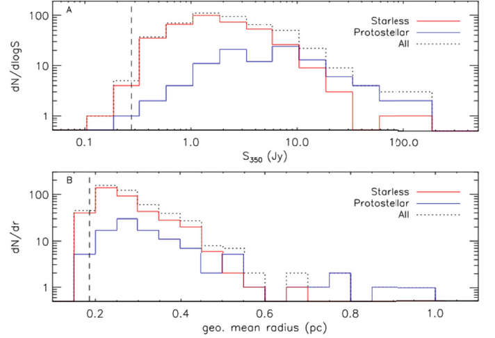
Fig. 2. Distributions of 350 \mu\text{m} fluxes (A) and geometric mean sizes (B) of RMC clumps. Dotted black, solid red, and solid blue lines indicate all clumps, starless clumps, and protostellar clumps, respectively. In panel A, the vertical dashed line indicates roughly a 3\sigma rms limit for detected clumps. In panel B, the vertical dashed line indicates the resolution limit of the smoothed 250 \mu\text{m} data.
