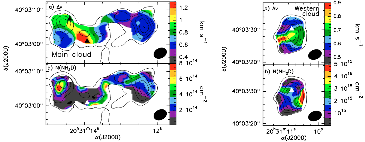
Fig. 2. Color-scale maps of linewidth and N(\text{NH}_2\text{D}) overlaid on the \text{NH}_2\text{D } 1_{11}-1_{01} integrated emission (contours) for the main cloud (left panels) and the western cloud (right panels). Triangles mark the \text{NH}_3 column density peaks of BIMA 3, BIMA 4 (left), and the western cloud (right). In all panels the synthesized beam is shown in the bottom right corner.
