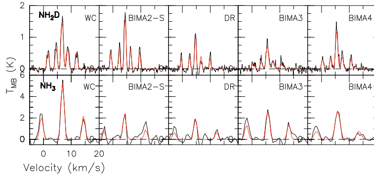
Fig. 3. Spectra (black line) toward 5 positions of the IRAS 20293+3952 for \text{NH}_2\text{D } 1_{11}-1_{01} (top) and \text{NH}_3 (1, 1) (bottom). The 5 positions, which are labeled in the top right corner of each panel, are, from left to right WC (western cloud), BIMA 2-S, DR (dust ridge core), BIMA 3, and BIMA 4. The red lines show the fit to the hyperfine structure obtained as illustrated in Sect. 3.
