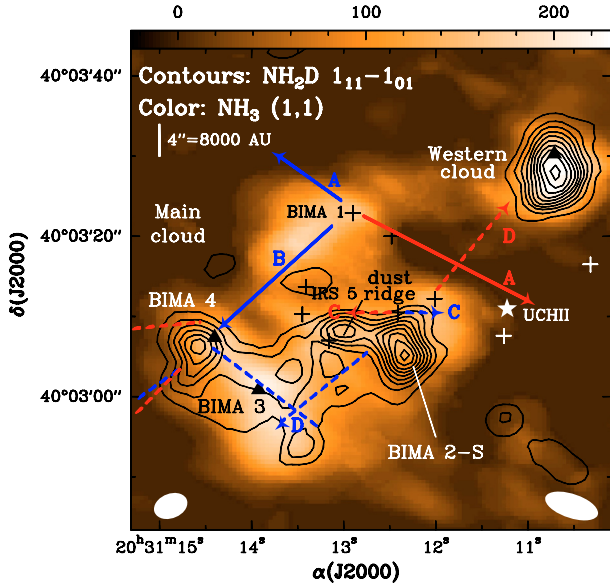
Fig. 1. Contours: \text{NH}_2\text{D} zero-order moment. Contours start at 6%, increasing in steps of 10% of the peak intensity, 0.58 \text{ Jy beam}^{-1} \text{ km s}^{-1} . Color scale: \text{NH}_3(1, 1) zero-order moment (Palau et al. 2007). The \text{NH}_2\text{D} synthesized beam, 4''.32 \times 3''.05 (PA = 111^\circ ), and the \text{NH}_3 synthesized beam are shown in the bottom left and bottom right corners, respectively. White star: position of the UCH II region (IRAS 20293+3952). Plus signs: YSOs embedded in the main cloud. Black triangles: \text{NH}_3 column density peaks in the starless cores BIMA 3, BIMA 4, and the western cloud. Main cores of \text{NH}_2\text{D} are labeled as western cloud, dust ridge, BIMA 2-S, and BIMA 4. The blue and red continuum/dashed arrows mark the direction of powerful/less powerful molecular outflows, respectively (Beuther et al. 2004a). Outflow B is deflected by BIMA 4 (Palau et al. 2007) and the dashed lines indicate the high-velocity gas around BIMA 4.
