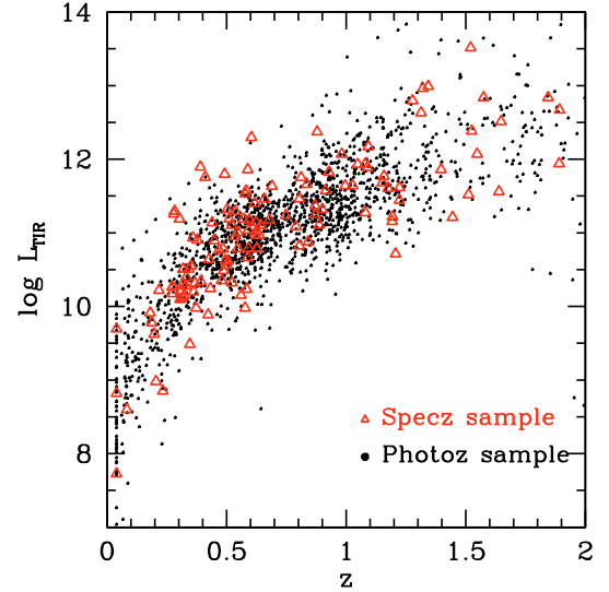
Fig. 12. TIR luminosity is shown as a function of photometric redshift. The photo- z is estimated using UV-optical-NIR photometry. L_{\text{TIR}} is obtained through SED fit in 7\text{--}24 \mu\text{m} .
