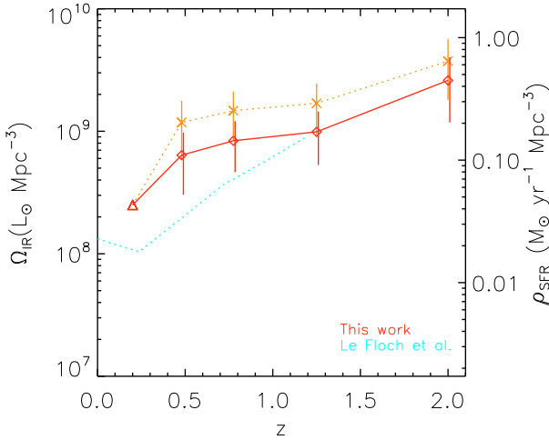
Fig. 5. Evolution of TIR luminosity density computed by integrating the 8 \mu\text{m} LFs in Fig. 4. The red solid lines use the conversion in Eq. (4). The orange dashed lines use Eq. (3). Results from Le Floch et al. (2005) are shown with the cyan dotted lines.
