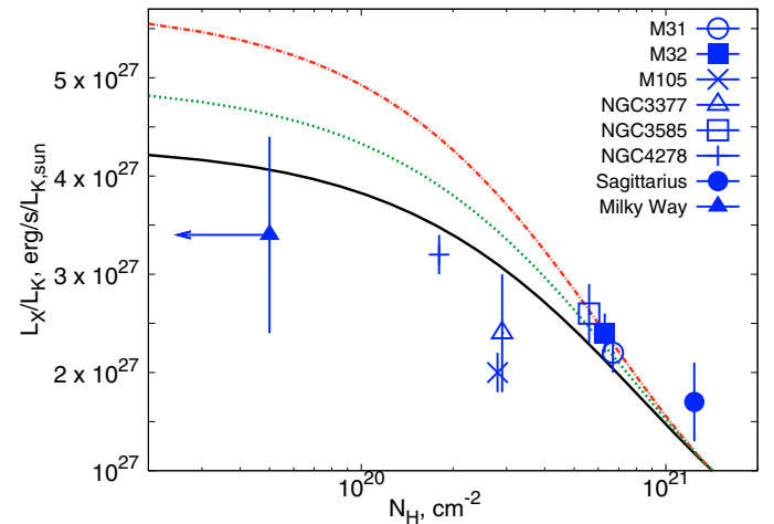
Fig. 4. The sensitivity-corrected L_X/L_K ratio versus Galactic hydrogen column density. The solid line (black) shows the dependence of the absorbed flux on the N_{\text{H}} assuming a power-law emission spectrum with slope \Gamma = 2 . The dotted line (green in the color version of this plot) and the dashed-dotted line (red) correspond to the combination of the same power-law with a blackbody spectrum with kT_{\text{bb}} = 75 \text{ eV} and kT_{\text{bb}} = 50 , respectively. For the last two curves equal luminosities of the two components in the 0.3–0.7 keV band was assumed. Milky Way represents the absorption-free L_X/L_K ratio, and its N_{\text{H}} value is shown as an upper limit and is arbitrarily placed along the x -axis.
