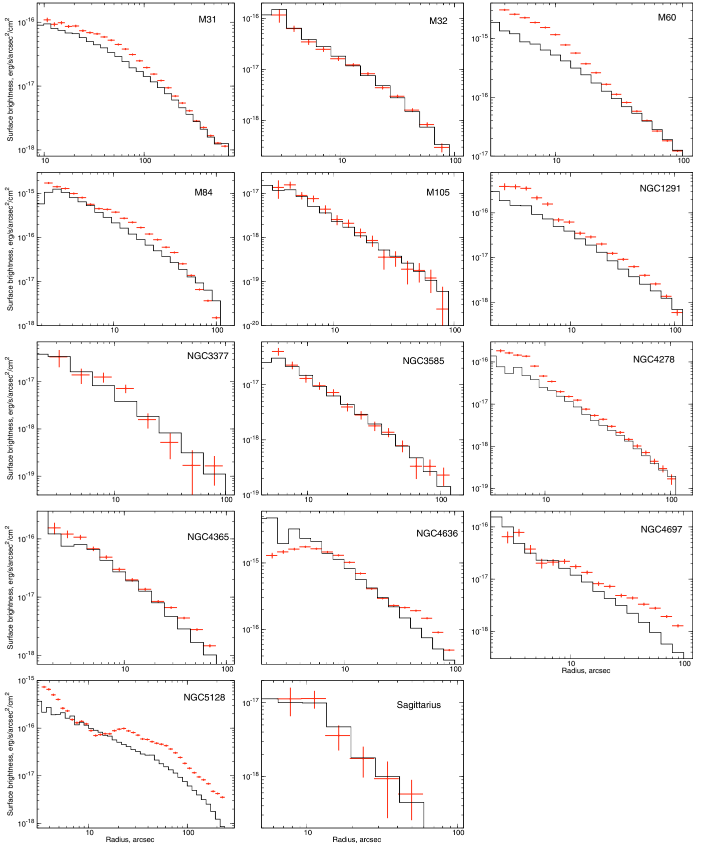
Fig. 1. Surface brightness profiles of the 14 galaxies in our sample in the 0.5–2 keV energy range. All background components were subtracted. Crosses (red) show the distribution of unresolved X-ray emission based on Chandra data, the solid line (black) shows the (arbitrarily) re-normalized near-infrared brightness.
