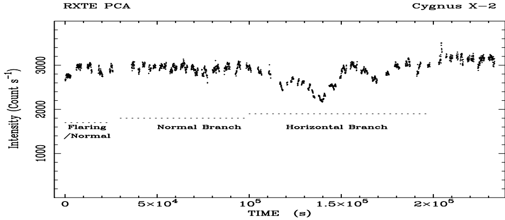
Fig. 1. Background-subtracted and deadtime-corrected PCA light curve of Cygnus X-2 with 64 s binning.
