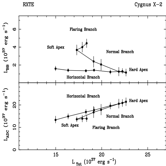
Fig. 4. Luminosities of the continuum emission components: neutron star blackbody emission ( upper panel ) and ADC Comptonized emission ( lower panel ).
