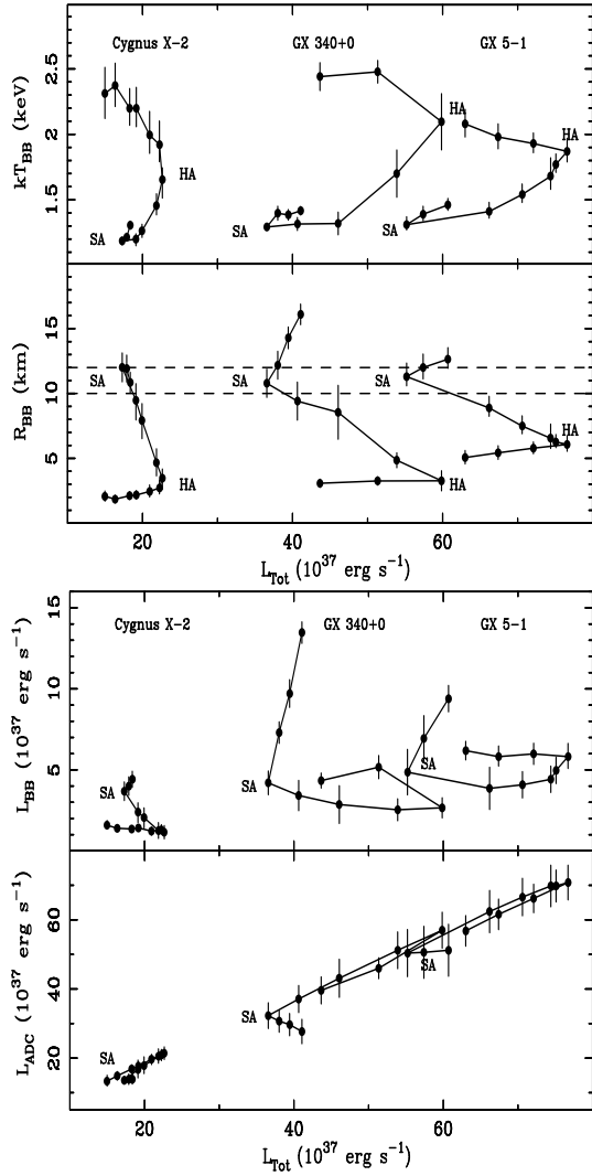
Fig. 5. Upper panel: blackbody temperature ( upper panel ) and radius ( lower panel ) as a function of the total luminosity; lower panel: the individual luminosities of the neutron star blackbody ( upper panel ) and of the Comptonized ADC emission as a function of the total luminosity ( lower panel ). The soft apex (SA) and hard apex (HA) are marked.
