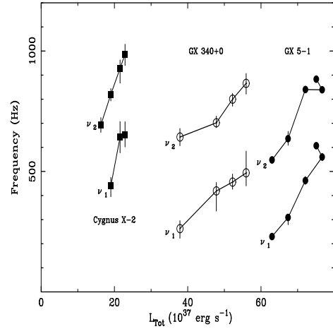
Fig. 9. Kilohertz QPO frequencies as a function of source luminosity for Cygnus X-2, GX 340+0 and GX 5-1.
