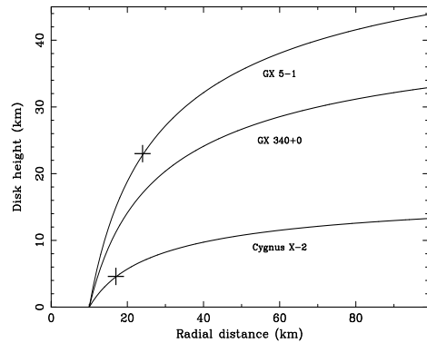
Fig. 11. Inner disk height profiles H(r) for the three sources with points indicating the position of the inner disk edge in GX 5-1 and Cygnus X-2 for f/f_{\text{Edd}} = 1.3 (see text).
