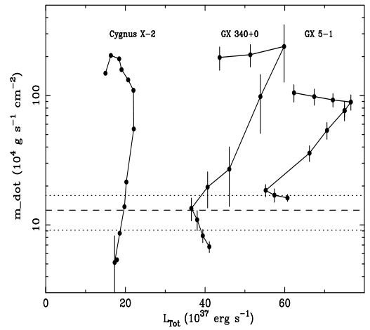
Fig. 7. Mass accretion rate per unit neutron star emitting area \dot{m} .
