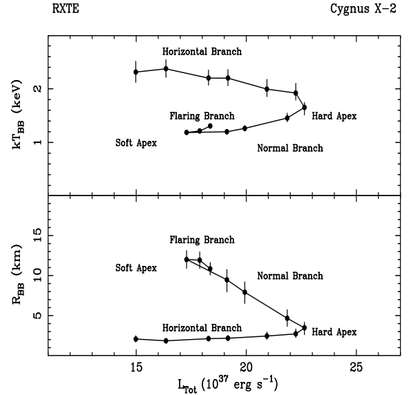
Fig. 3. Left: blackbody temperature (upper panel) and radius (lower panel) as a function of the total luminosity.
