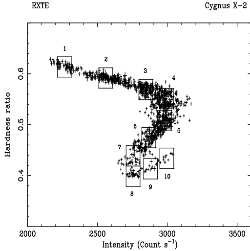
Fig. 8. Selection boxes used for fitting of the power spectra.
