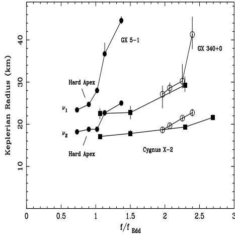
Fig. 10. Keplerian radial positions corresponding to the upper kHz QPO ( \nu_2 ) and lower kHz QPO ( \nu_1 ) as a function of the strength of the neutron star radiation pressure expressed as f/f_{\text{Edd}} (see text).
