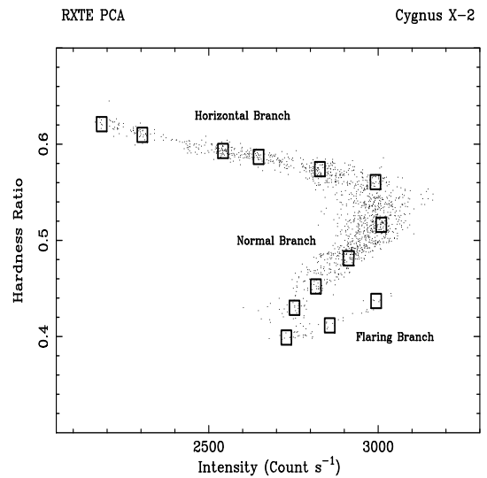
Fig. 2. Hardness ratio (7.3–18.1 keV)/(4.1–7.3 keV) variation with intensity.
