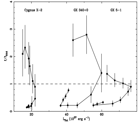
Fig. 6. Flux of the emitting part of the neutron star as a fraction of the Eddington flux (assumed constant) L_{\text{Edd}}/4\pi R^2 , where R = 10 km.
