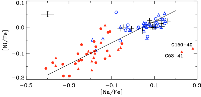
Fig. 2. [Ni/Fe] versus [Na/Fe] with the same symbols as in Fig. 1. The linear fit does not include the two Na-rich stars.
