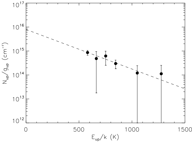
Fig. 5. Rotation diagram for the CO lines observed towards VY CMa. The dashed line is a fit to the 4 lowest energy lines using the manually fitted fluxes from Table 5.
