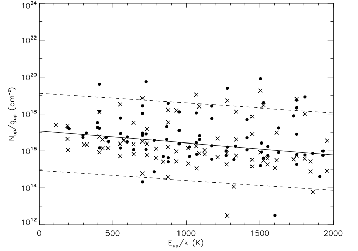
Fig. 4. Rotation diagram resulting from fit to water lines in the LWS spectrum of VY CMa weighted by A_{ul} and E_u . Ortho water lines are shown as filled circles and para water lines as crosses. The best fit to lines with upper state energies less than 2000 K (ignoring outlying points) is shown, giving a rotational temperature of 670_{-130}^{+210} K.
