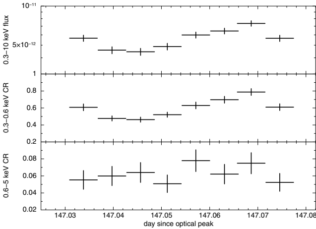
Fig. 3. The top panel shows the V598 Pup XMM-pn flux light-curve (0.3–10 keV, unabsorbed in erg cm -2 s -1 ), while the middle and bottom panels show the soft (0.3–0.6 keV) and hard (0.6–5 keV) count-rate light-curves respectively, in units of count s -1 . Note the different scales of the lower two panels.
