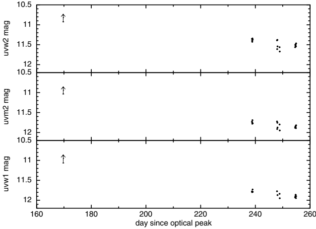
Fig. 5. Swift-UVOT light-curves of V598 Pup in the UV filters. The observations on day 169 are lower limits only, because the source was bright enough to saturate the detector. The horizontal bar at the bottom of each arrow indicates the limit on the magnitude.
