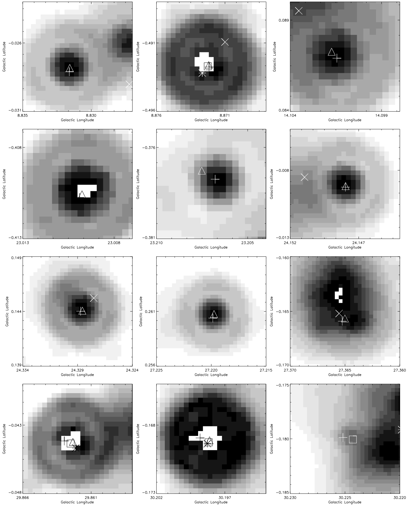
Fig. 6. Gray scale is the MIPS GAL 24\ \mu\text{m} emission, the pluses are the positions of 6.7-GHz methanol masers, the triangles are the positions of GLIMPSE point sources, the squares are the positions of 2MASS point sources, the stars are the positions of MSX point sources, and the crosses are the positions of IRAS point sources. Moving from the top left to the bottom right, the sources are G8.8316-0.0281, G8.8722-0.4928, G14.1014+0.0869, G23.0099-0.4107, G23.2068-0.3777, G24.1480-0.0092, G24.3287+0.1440, G27.2198+0.2604, G27.3652-0.1659, G29.8630-0.0442, G30.1987-0.1687, G30.2251-0.1796, G30.8987+0.1616, 18556+0136, G43.15+0.02, 19120+0917, 19186+1440, and W51e2.
