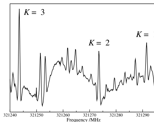
Fig. 2. Section of the lower submillimeter spectrum of CH 3 CN. Transitions of ^{13}\text{CH}_3^{13}\text{CN} have been labeled with their K quantum numbers. This isotopolog is less abundant by a factor of 8000 compared to the main isotopolog. While the spectrum is rather sparse on the level of the strongest CH 3 CN transitions, it is considerably less sparse on the level of the CH 3 C 15 N transition, see Fig. 1, and rather dense on the level of the ^{13}\text{CH}_3^{13}\text{CN} transitions. One of the lines may be due to a high- K , \nu_8 = 1 line of ^{13}\text{CH}_3\text{CN} , all other transitions remain unassigned, see Sect. 3.5.
