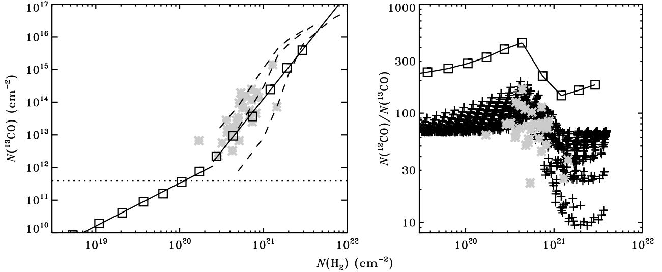
Fig. 8. Column densities of ^{13}\text{CO} (left) and column density ratios of ^{12}\text{CO} to ^{13}\text{CO} (right) plotted against the column density of \text{H}_2 . Grey crosses: observations of Sonnentrucker et al. (2007) , Burgh et al. (2007) and Sheffer et al. (2007) . Black squares and straight lines: 100-point means from our grid of translucent cloud models, offset by a factor of three in the right panel. Dotted line: median depth at which ^{12}\text{CO} becomes self-shielding. Black plus signs: model data for all points with A_V \leq 5 mag. Dashed lines: data from the translucent cloud models of vDB88 for \chi = 0.5, 1 and 10 (left to right).
