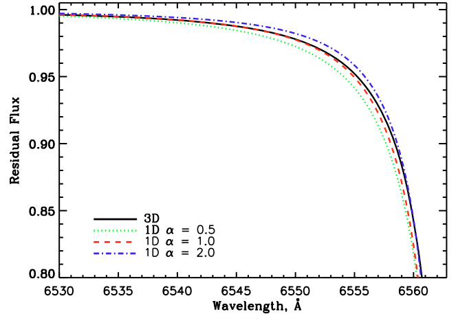
Fig. 1. H \alpha Balmer line profiles computed using a 3D model and 1D models with varying mixing-length parameter \alpha , for T_{\text{eff}} = 5920 K, \log g = 4.50 and [Fe/H] = -3.00.
