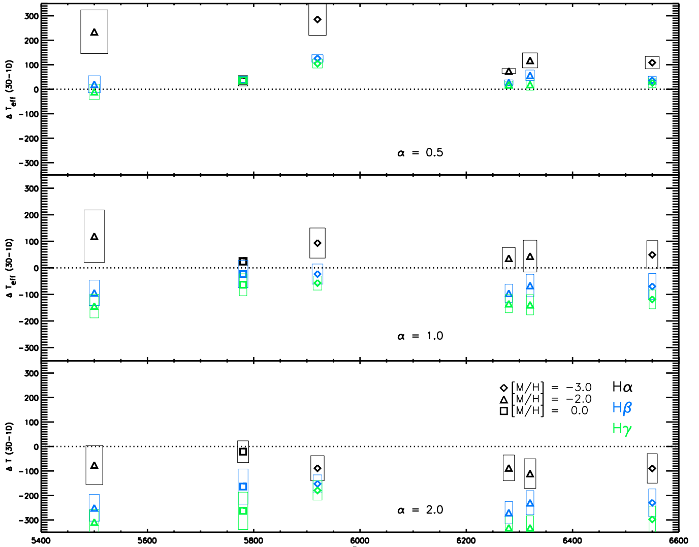
Fig. A.1. The temperature differences (3D – 1D) using 1D models with \alpha = 0.5 , \alpha = 1.0 and \alpha = 2.0 , for H\alpha , H\beta , and H\gamma for all of the six models considered. The uncertainties related to each temperature difference measurement are displayed as boxes. The value of the uncertainty on the x-axis corresponds to the associated \sigma_{T_{\text{eff}}} (sensitivity) values, while the uncertainty on the y-axis corresponds to the associated QF (quality of fit) values. See Table 2 and the text for details.
