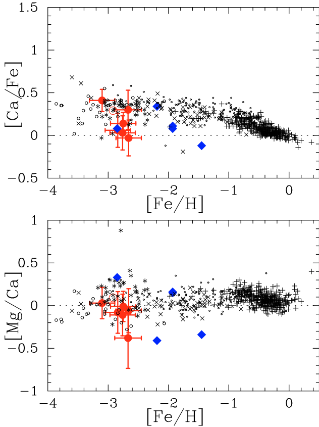
Fig. 3. The same as Fig. 2, but for [\text{Ca}/\text{Fe}] (top) and [\text{Mg}/\text{Ca}] (bottom).
