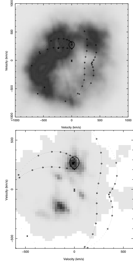
Fig. 3. Doppler maps of He II \lambda 4686 (top) and the Bowen complex (bottom). Indicated on both maps is the Roche lobe, gas stream leaving the L_1 point, and the Keplerian velocity along the stream for the assumptions q = 0.059 and K_2 = 275 \text{ km s}^{-1} .
