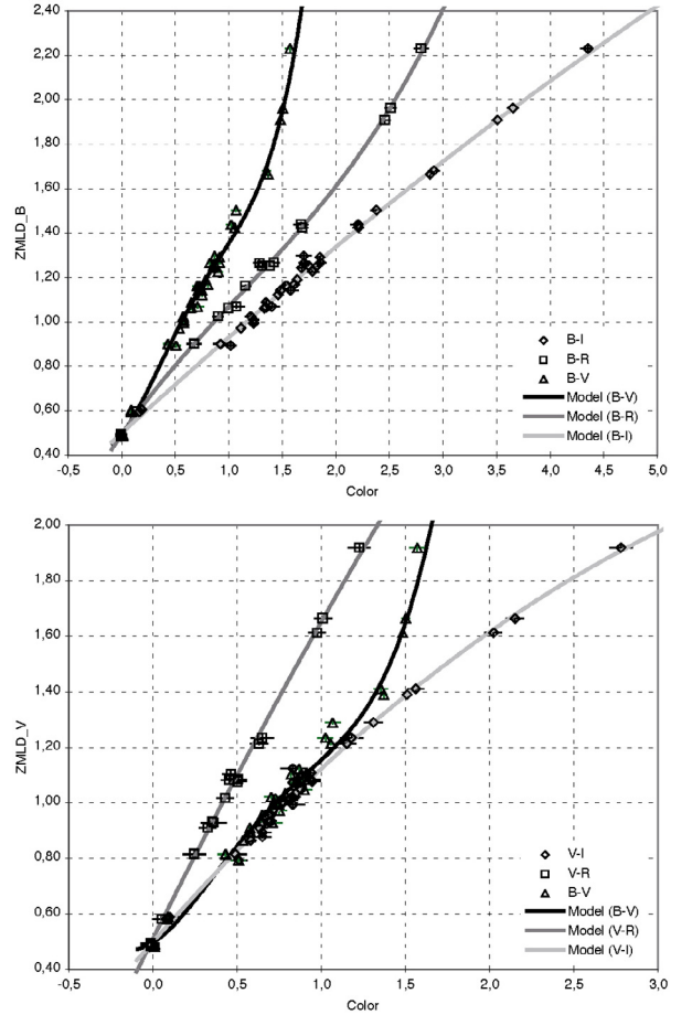
Fig. 1. Adjusted polynomial relations giving the zero-magnitude limb-darkened disk angular diameter ( ZMLD_\lambda ) in the B and V bands as a function of different color combinations. The corresponding polynomial coefficients are listed in Table 3.
