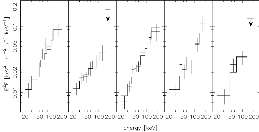
Fig. 1. Total-flux spectra of 4U0142+61 taken during INTEGRAL revolutions ( from left to right ); 142–189, 202–269, 331–336, 384–396 and 452–468. Data points are binned to 4\sigma if the single bins are of less significance. The upper limits represent 2\sigma confidence levels.
