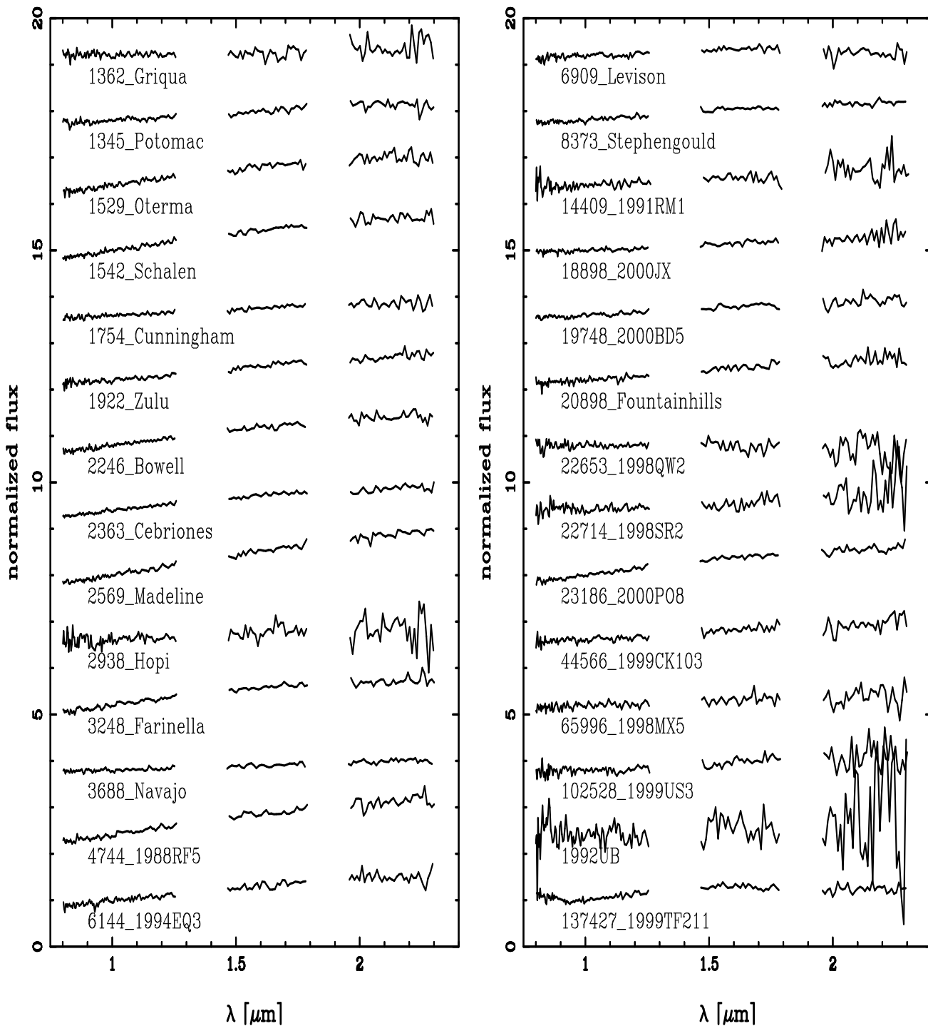
Fig. 1. Near-infrared reflectance spectra of the asteroids, normalized at 1.0 \mu\text{m} . Spectra are shifted in reflectance for clarity.
